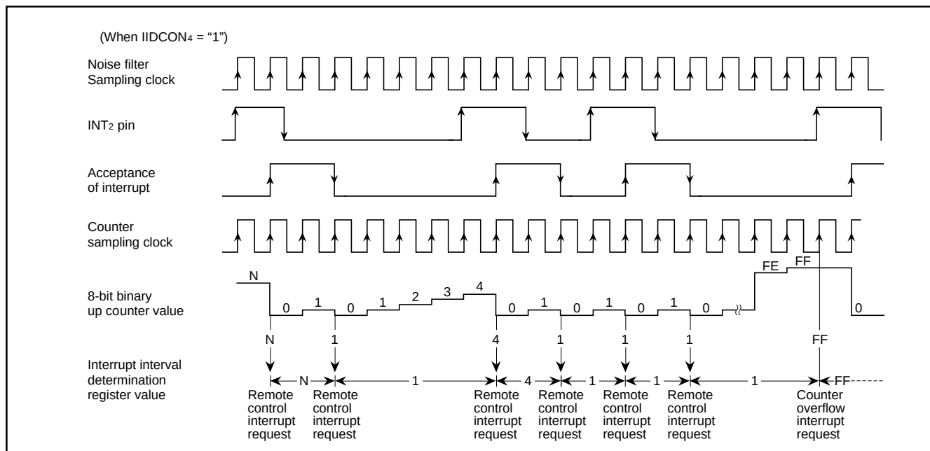
Fig. 38 Interrupt interval determination operation example (at both-sided edge active)
