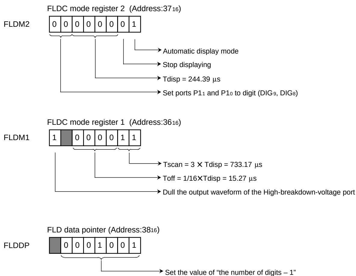
Fig. 2.5.14 Setting of related registers (1) [FLD automatic display and Key-scan using segment pin]
