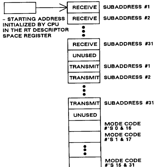
Figure 5. Descriptor Space
