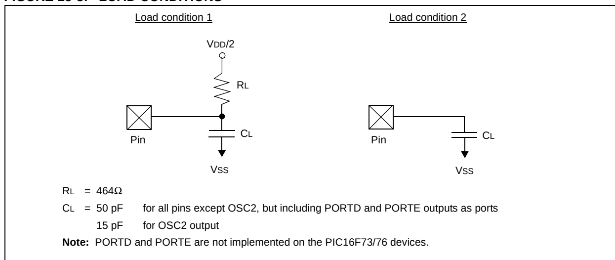
FIGURE 15-3: LOAD CONDITIONS
