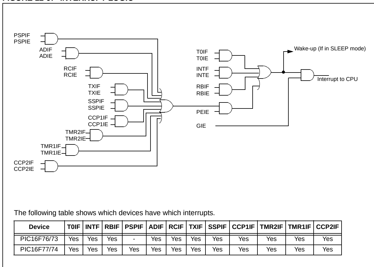
FIGURE 12-9: INTERRUPT LOGIC
