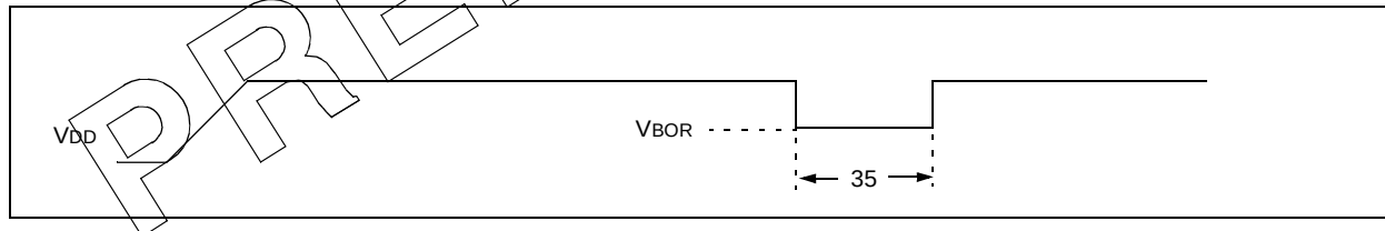
FIGURE 15-7: BROWN-OUT RESET TIMING
