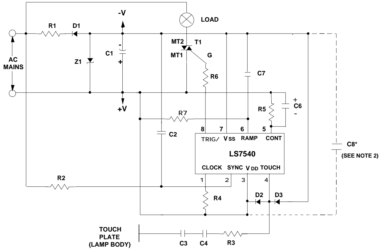
FIGURE 6. TOUCH LAMP APPLICATION SCHEMATIC #2
