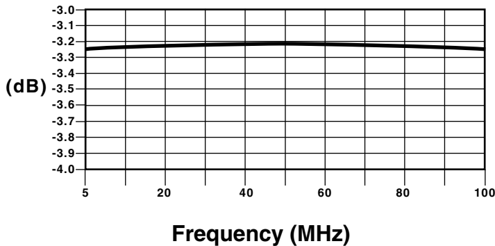
INSERTION LOSS
