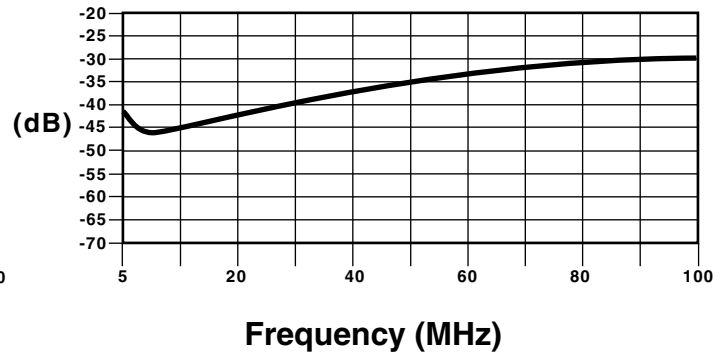
ISOLATION
