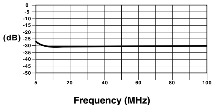
OUTPUT RETURN LOSS
