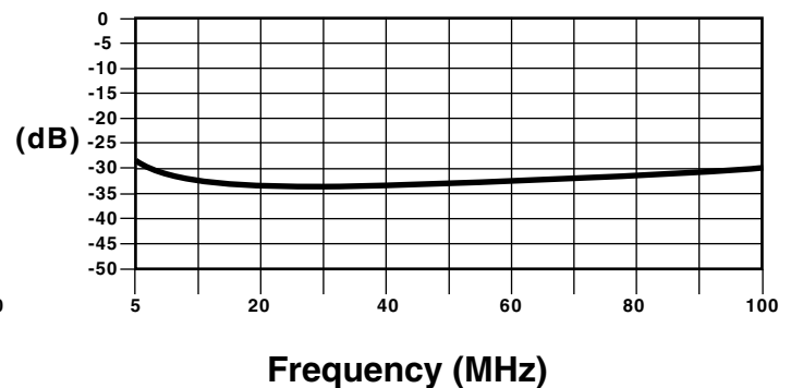
INPUT RETURN LOSS
