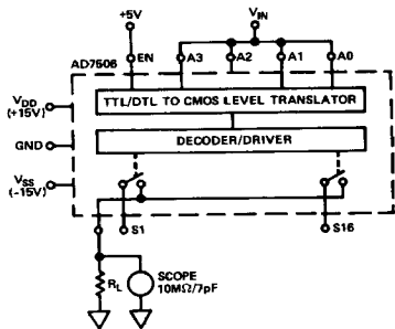
TEST CIRCUIT 1
