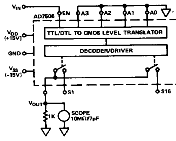
TEST CIRCUIT 2
