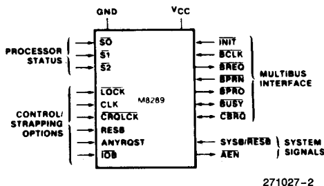
Figure 2. Functional Pinout
