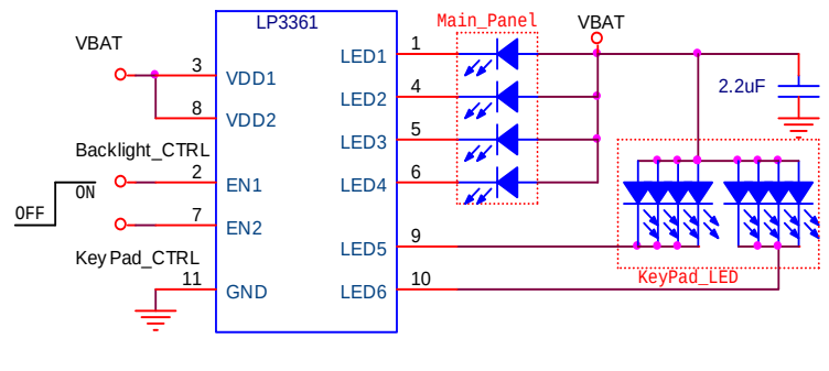
LP3361 Driver Panel and Keypad WLED Application
