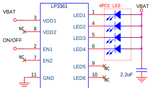
LP3361 Driver 4pcs White-LED Application
