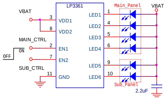
LP3361 Driver Dual Panel Application
