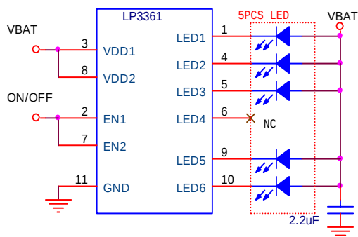
LP3361 Driver 5pcs White-LED Application
