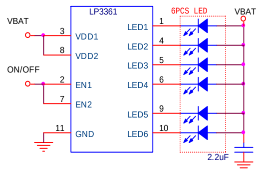
LP3361 Driver 6pcs White-LED Application
