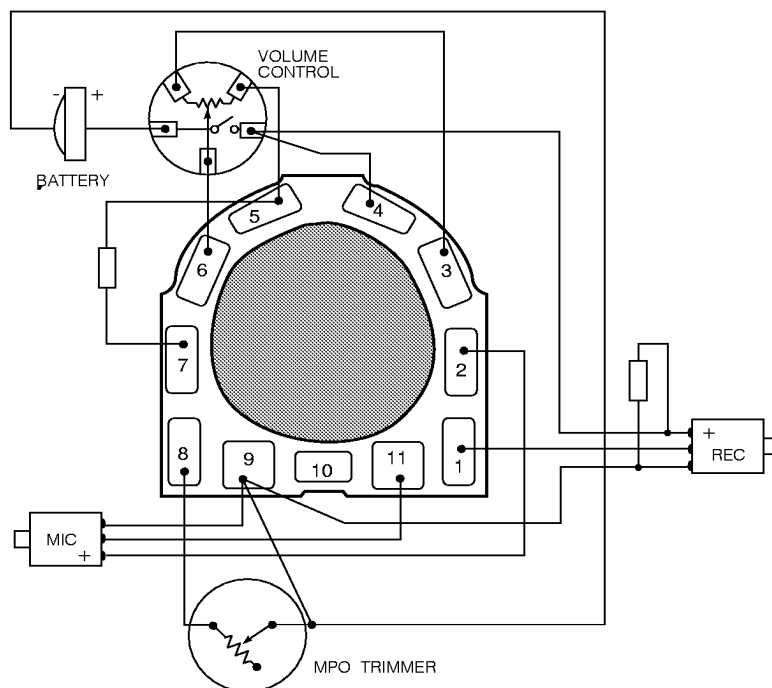
Fig. 12 Typical Assembly Diagram
