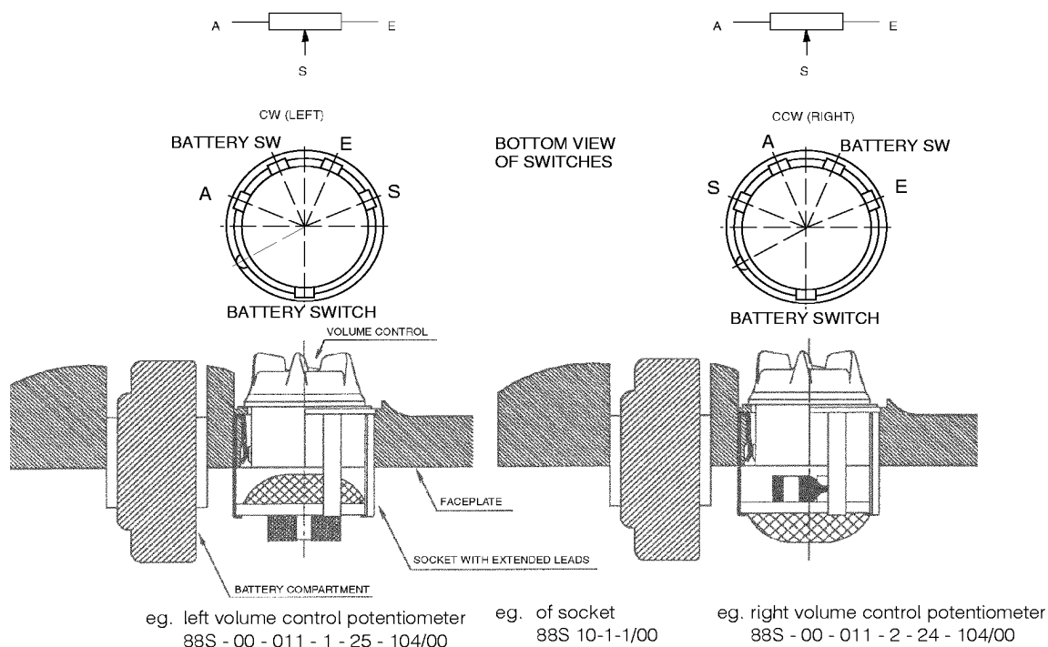
Fig. 11 Gennum Hybrid Concept with Microtronic PJ88S VC Socket
