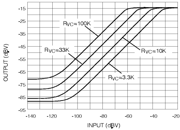
Fig. 3 I/O for Various R_{VC} Values
