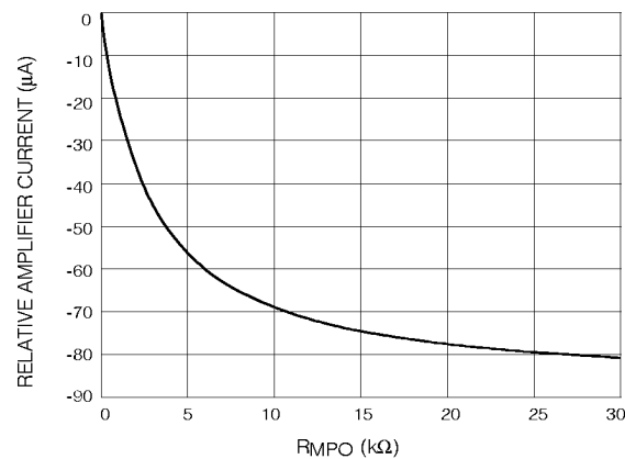
Fig. 7 Relative Amplifier Current vs MPO Resistance
