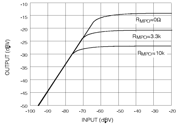
Fig. 4 I/O for Various R_{MPO} Values
