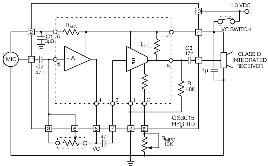
Fig. 2 Typical Hearing Instrument Application
