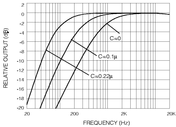
Fig. 5 Frequency Response for Various C_1/C_2 Values
