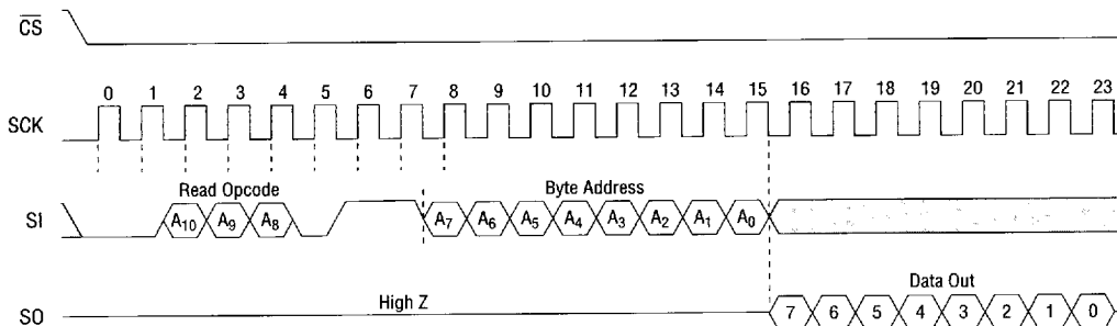
Figure 5. Read Sequence
