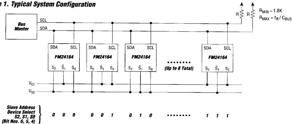
Figure 1. Typical System Configuration
