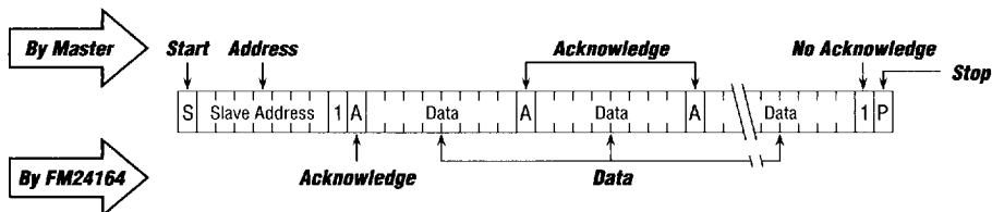
Figure 8. Sequential Read
