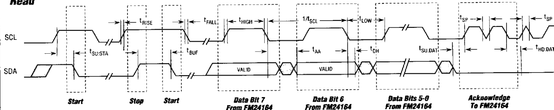
Figure 3. Bus Timing
