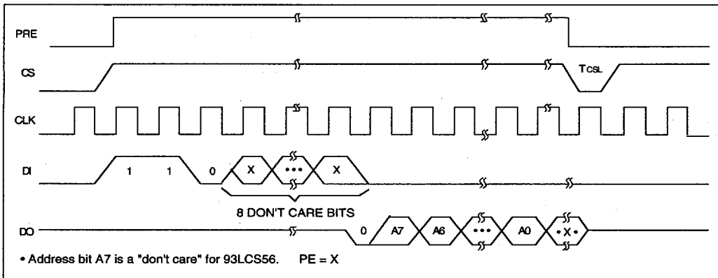
FIGURE 14-10: PREN TIMING
