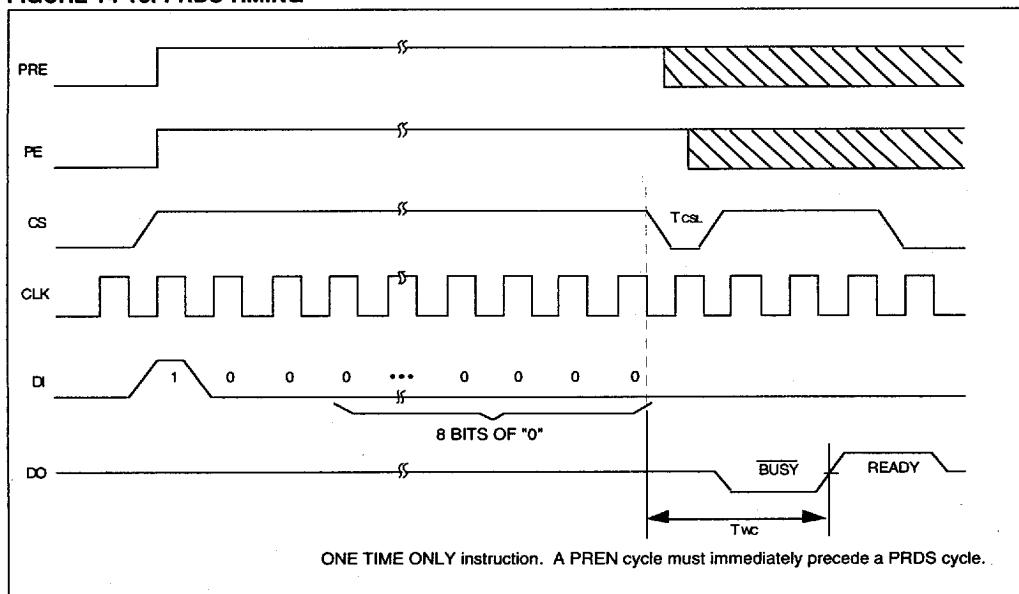
FIGURE 14-13: PRDS TIMING
