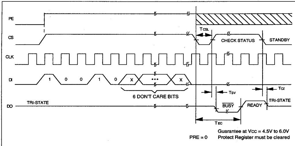
FIGURE 14-9: PRREAD TIMING
