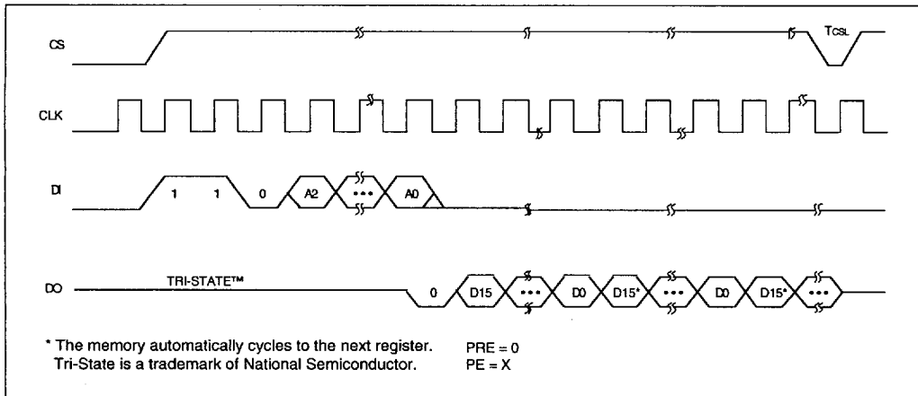
FIGURE 14-2: READ TIMING
