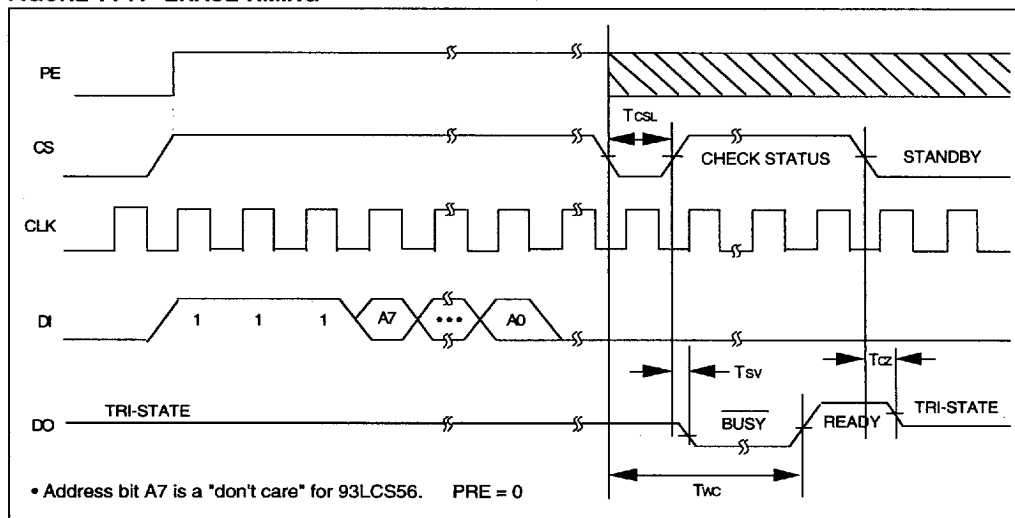
FIGURE 14-7: ERASE TIMING
