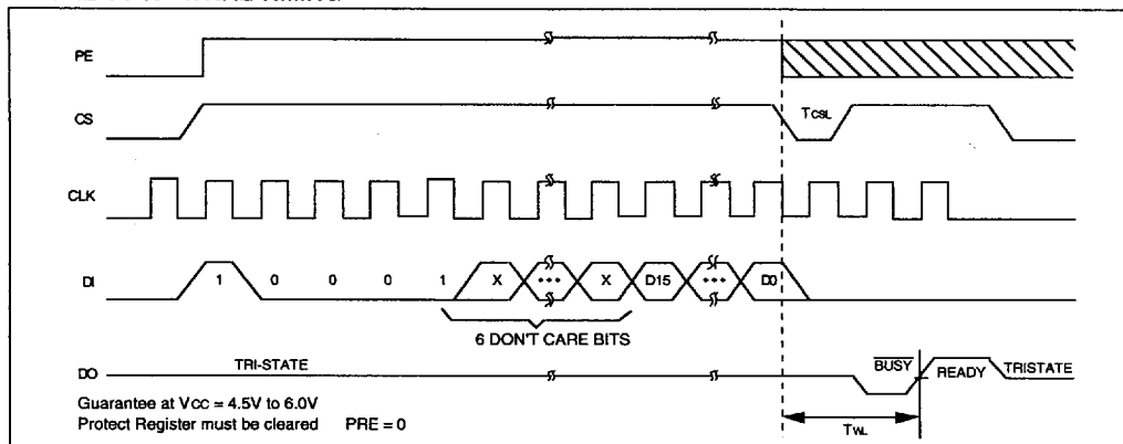
FIGURE 14-7: ERASE TIMING
