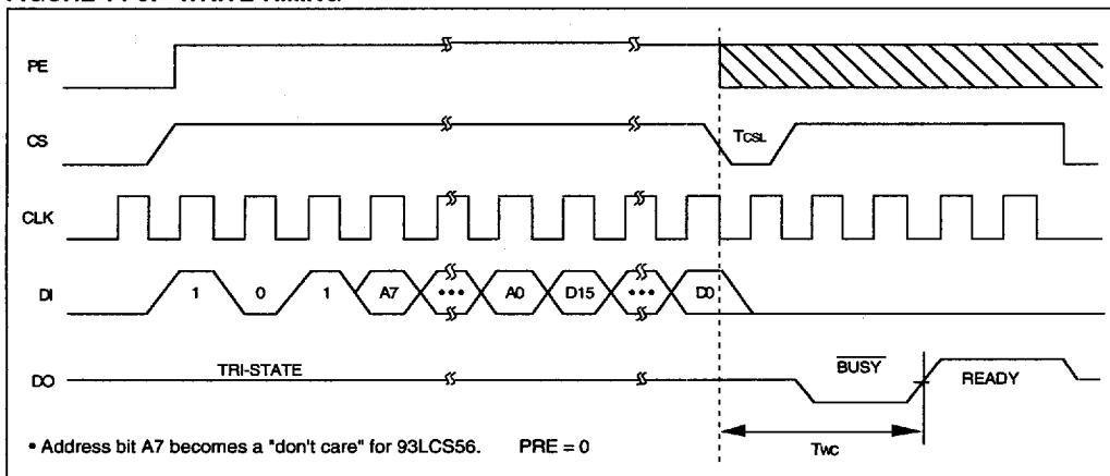
FIGURE 14-5: WRITE TIMING
