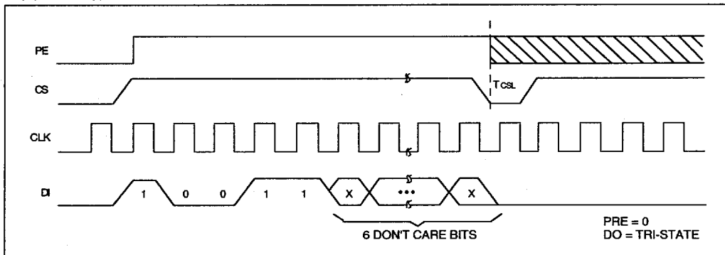
FIGURE 14-4: EWDS TIMING
