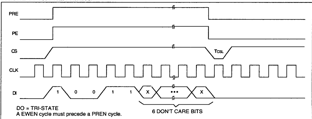
FIGURE 14-10: PREN TIMING
