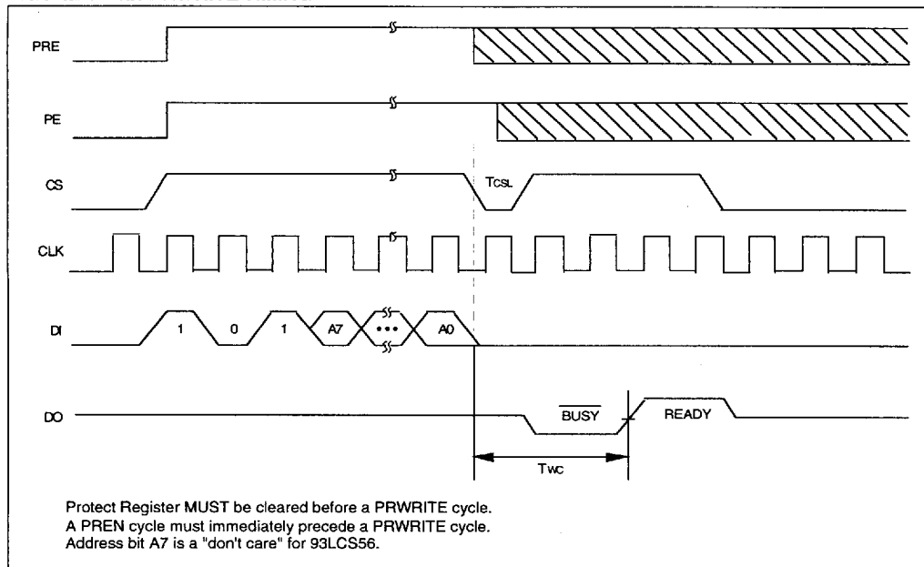
FIGURE 14-12: PRWRITE TIMING
