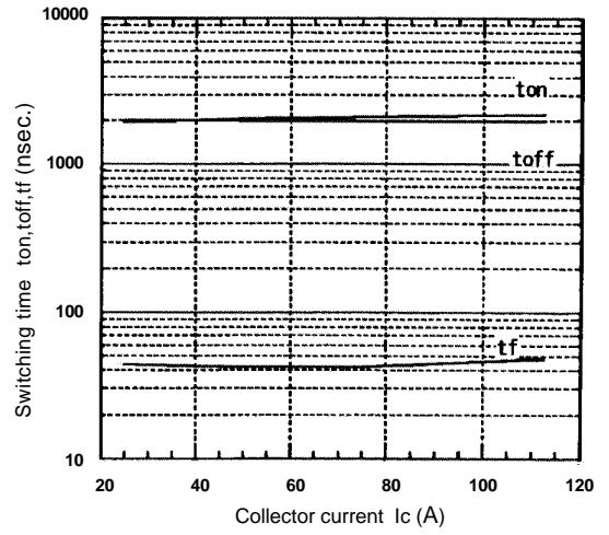
Switching time vs. Collector current Edc=300V, Vcc=15V, Tj=125°C
