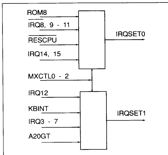
FIGURE 5-2. IRQSET - WHEN NOT IN STAND ALONE MODE
