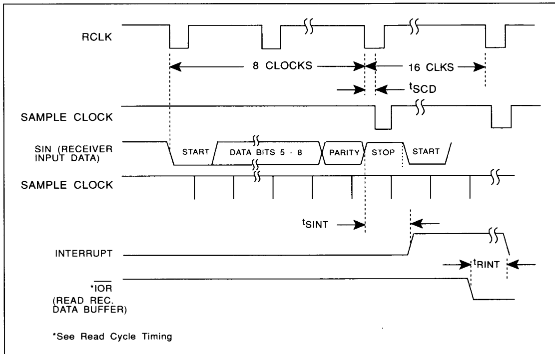
FIGURE 6-1. RECEIVER TIMING
