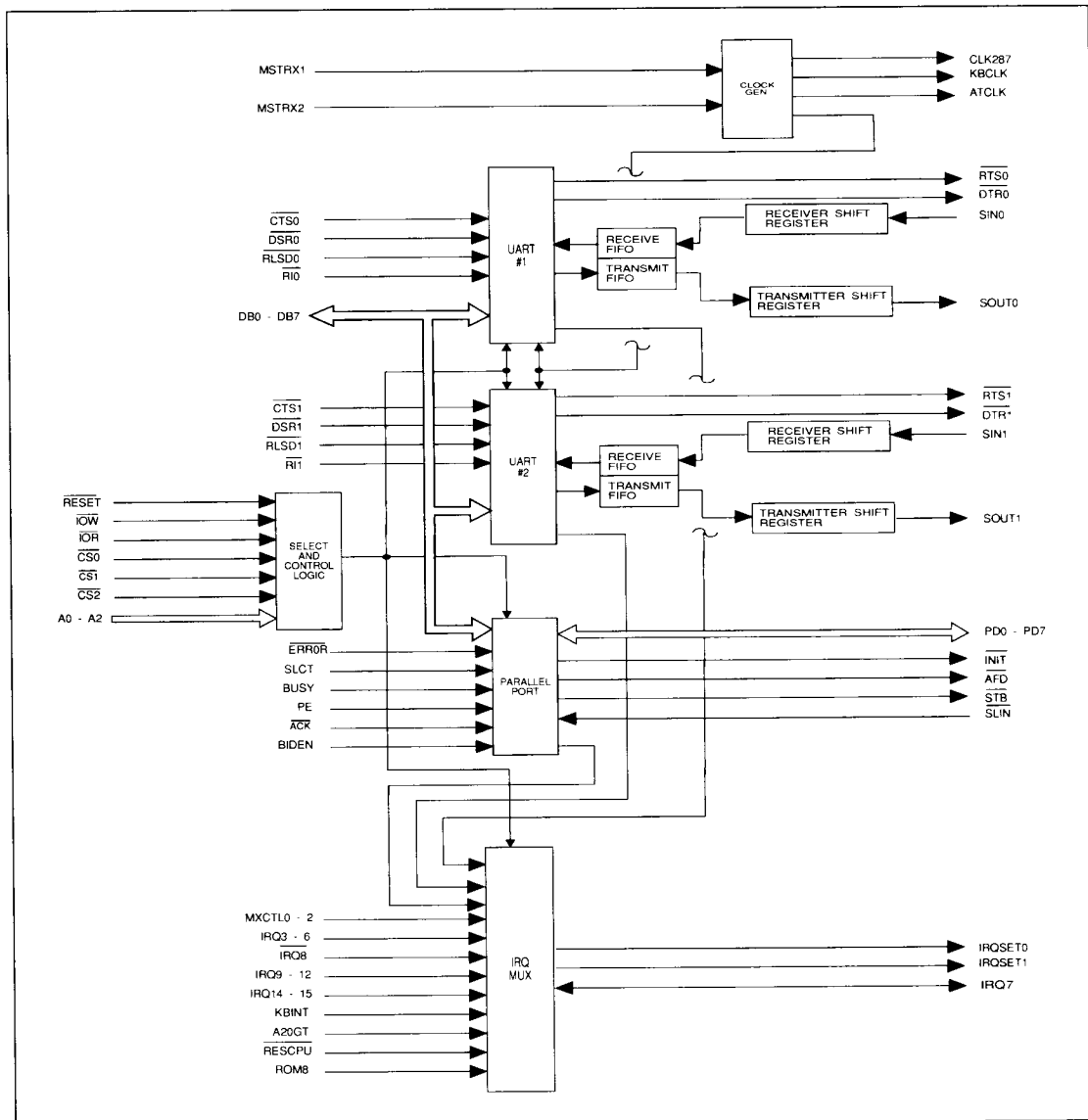
FIGURE 1-1. WD76C30 BLOCK DIAGRAM
