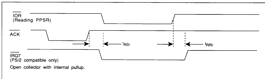
FIGURE 6-9. PARALLEL PORT INTERRUPT TIMING
