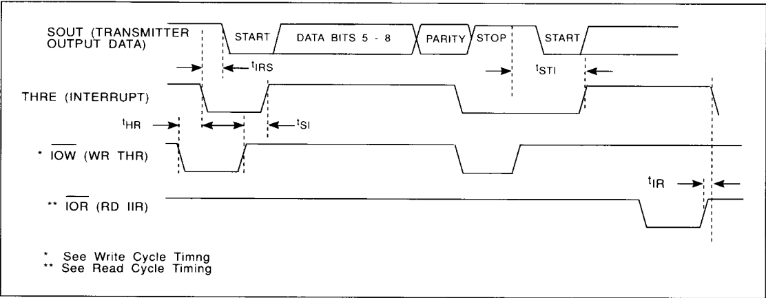
FIGURE 6-2. TRANSMITTER TIMING
