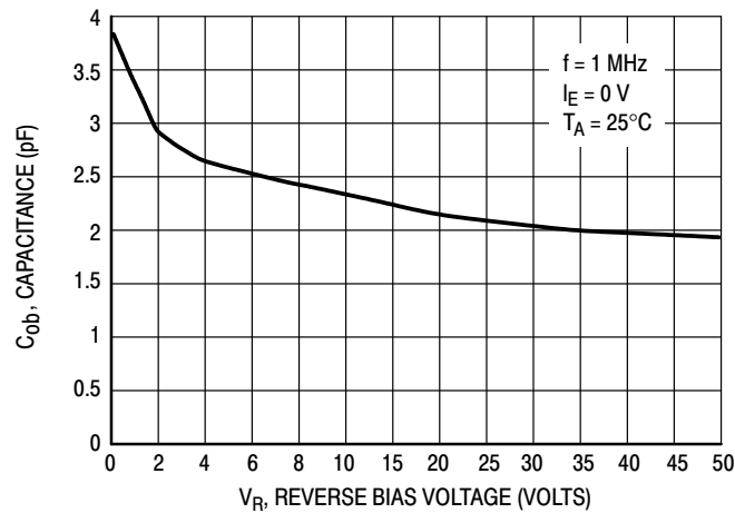
Figure 5. Output Capacitance
