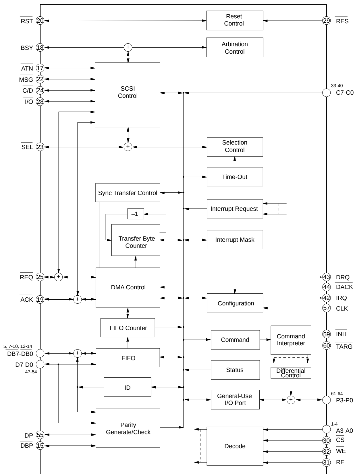
Block Diagram (CXD1185CQ)
