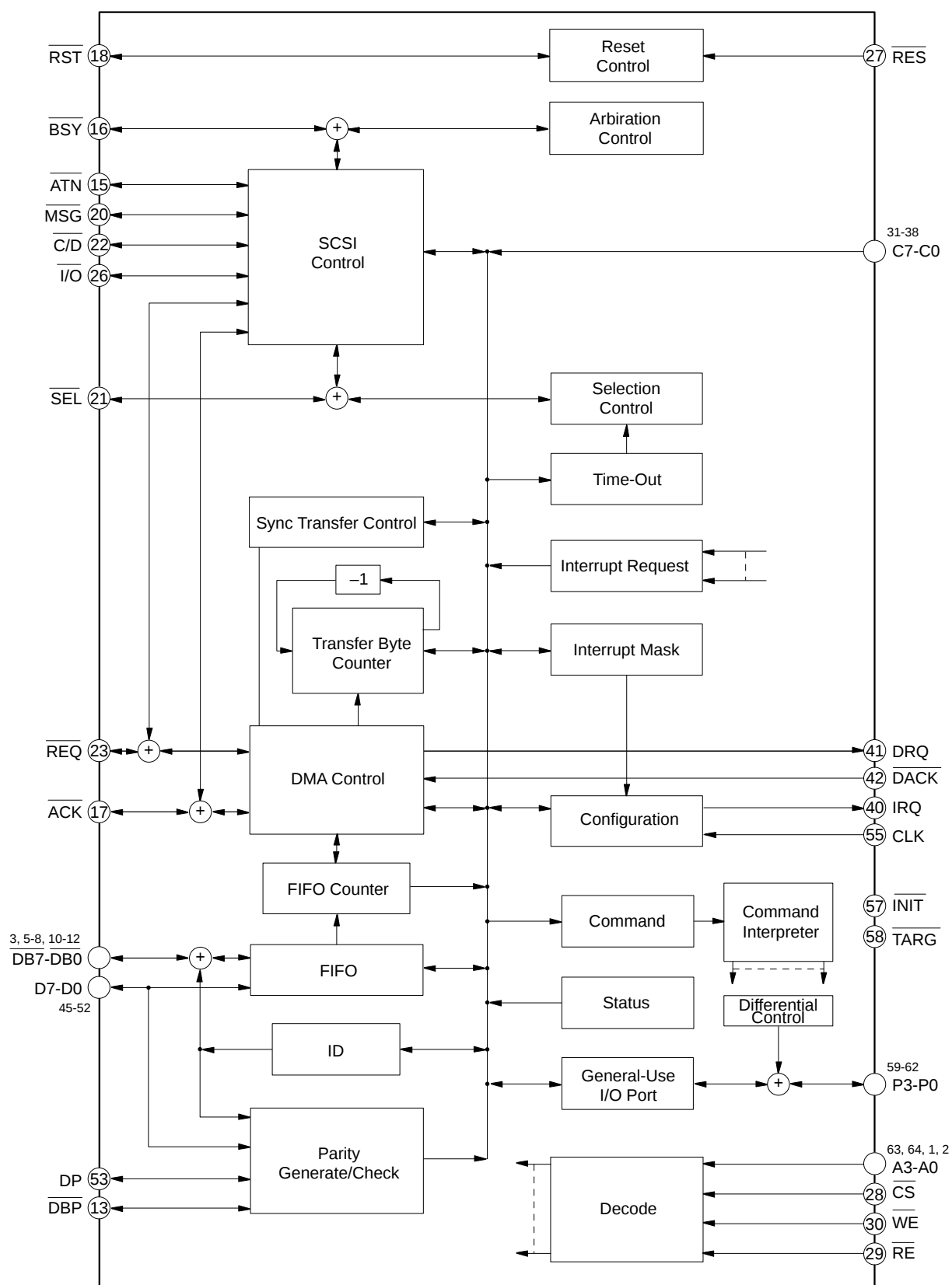
Block Diagram (CXD1185CR)
