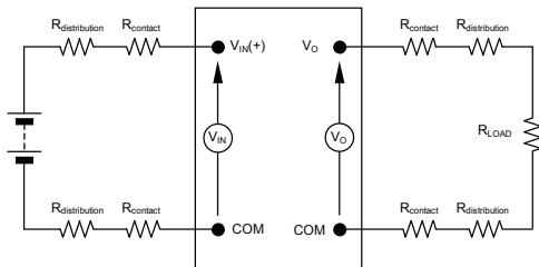
Figure 25. Output Ripple and Noise Test Setup.
