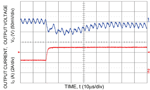
Figure 13. Transient Response to Dynamic Load Change from 50% to 100% of full load ( V_o = 5.0 Vdc , C_{ext} = 2 \times 150 \mu F Polymer Capacitors).
