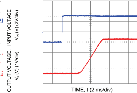
Figure 17. Typical Start-Up with application of V_{in} ( V_{in} = 5.0\text{ Vdc} , V_o = 3.3\text{ Vdc} , I_o = 5\text{ A} ).
