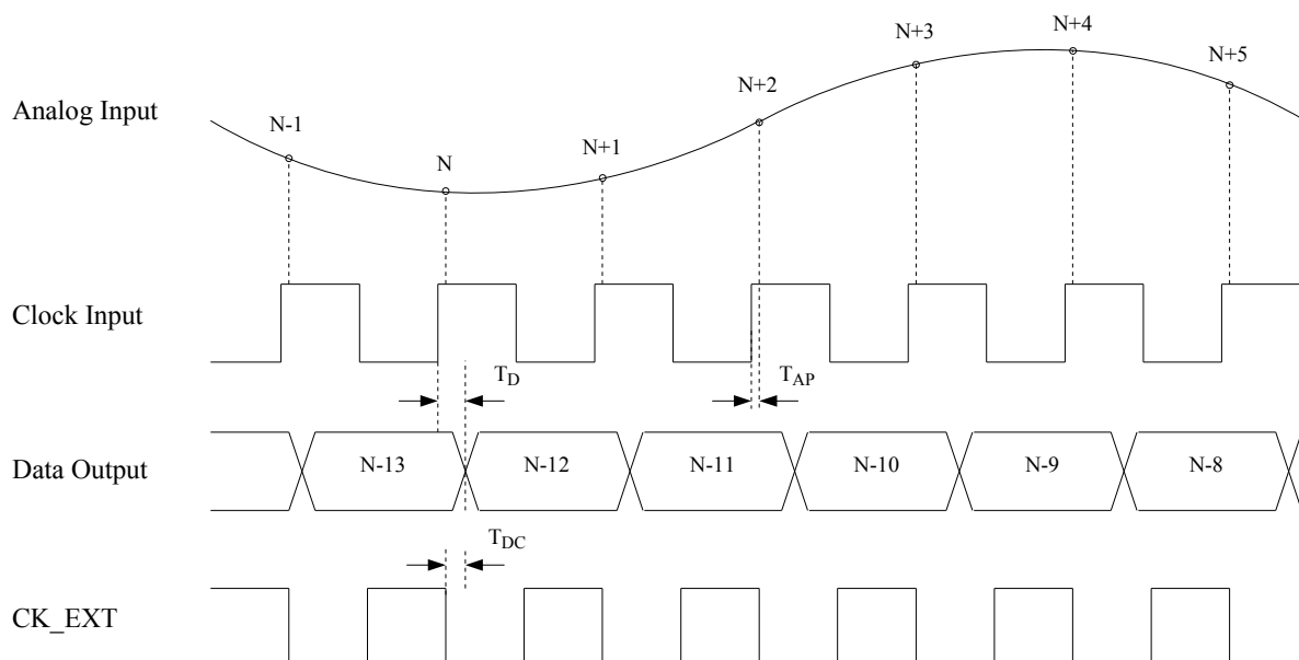
Figure 2: Timing Diagram
