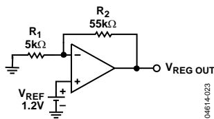
Figure 23. Voltage Regulator
