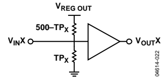
Figure 22. Gamma Buffers Tap Point Circuit
