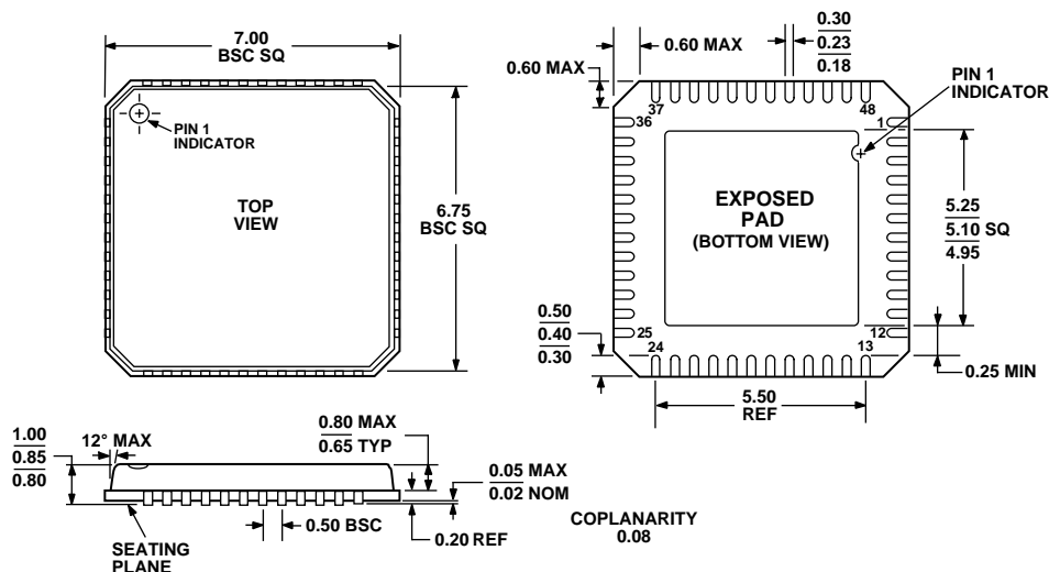
Figure 26. 48-Lead Lead Frame Chip Scale Package [LFCSP] 7 mm × 7 mm Body (CP-48)
