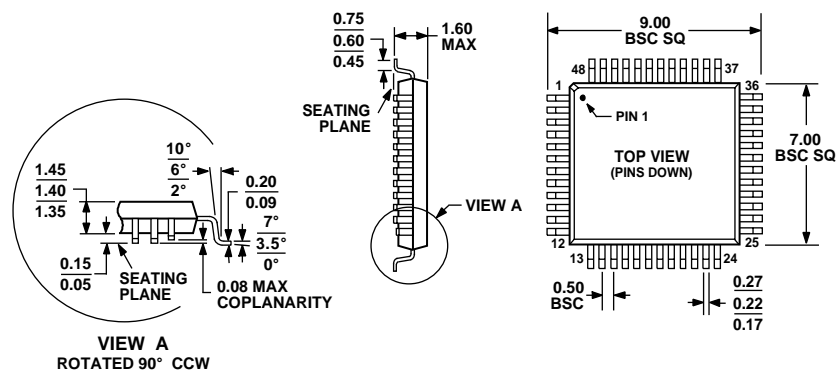
Figure 27. 48-Lead Low Profile Quad Flat Package [LQFP] (ST-48)
