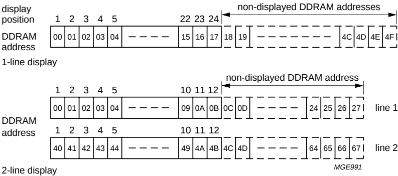
Fig.3 DDRAM to display mapping; no shift.
