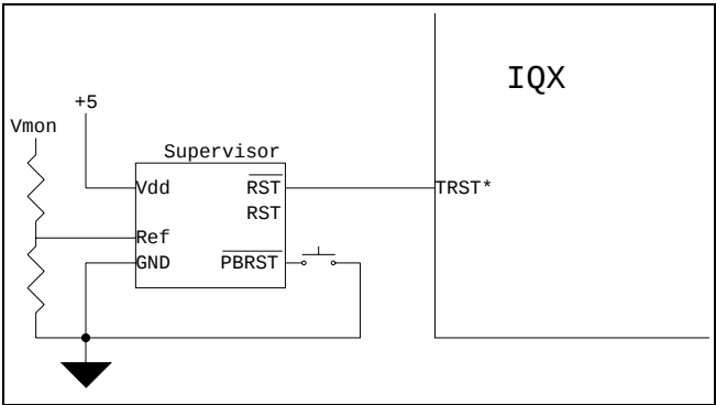
Figure 8. Reset Circuit
