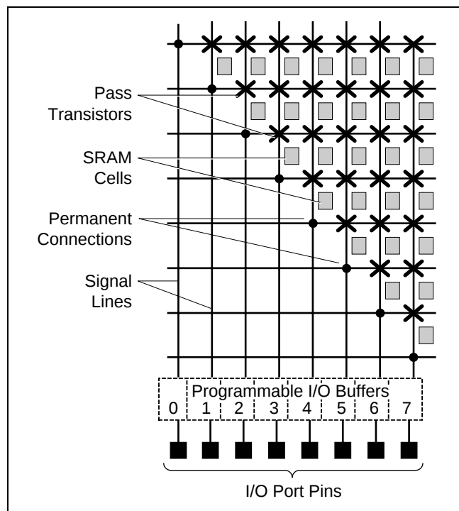
Figure 2. Switch Matrix Structure
