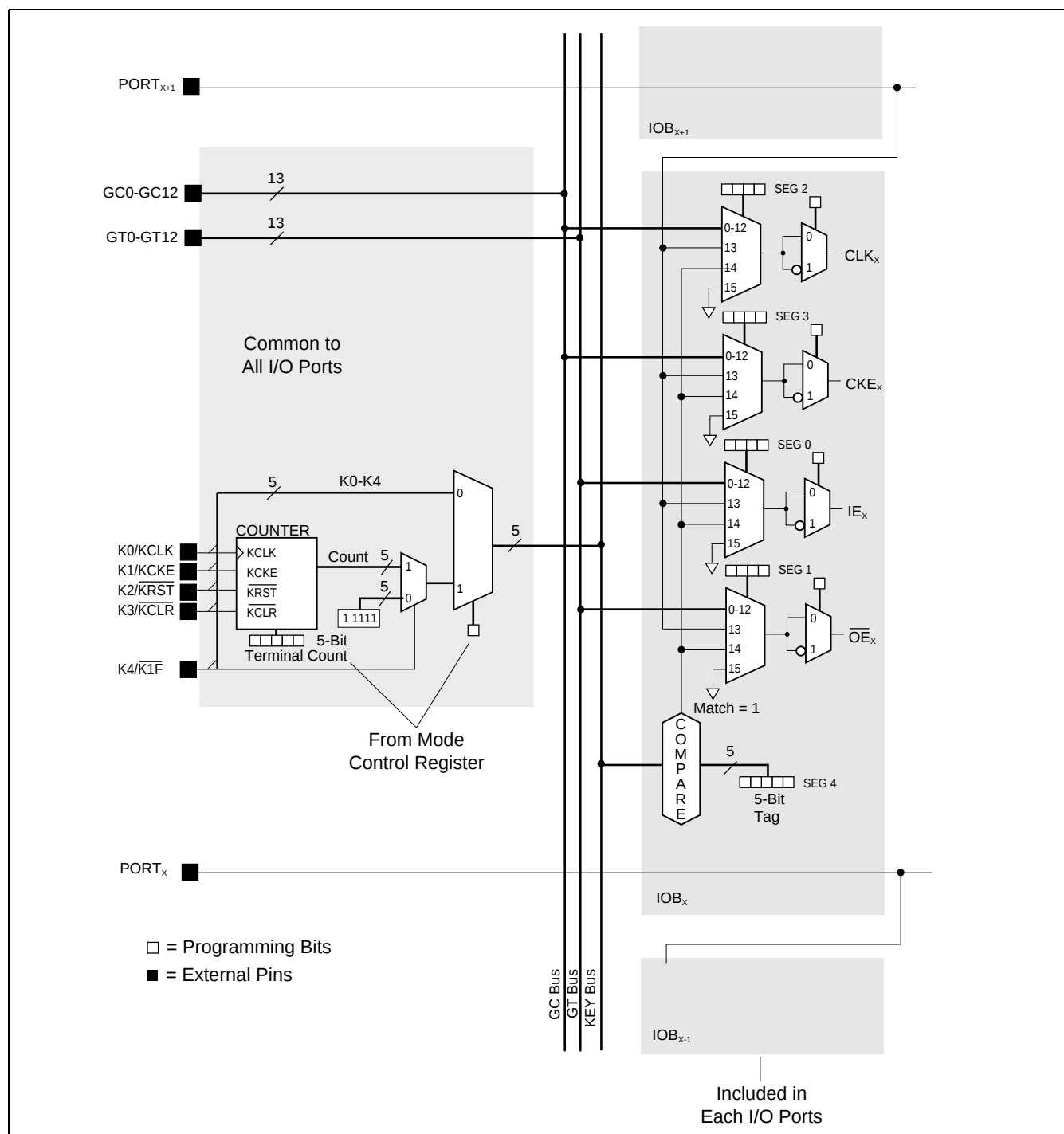
Figure 6. I/O Control
