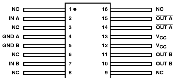
HS-4423RH, HS-4423BRH (FLATPACK CDFP4-F16) TOP VIEW
