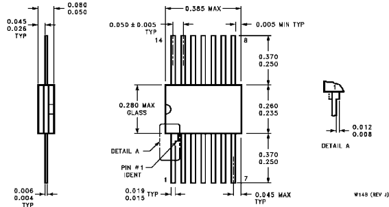
14-Lead Ceramic Flat Package (W) Order Number 5420FMQB or DM5420W NS Package Number W14B
