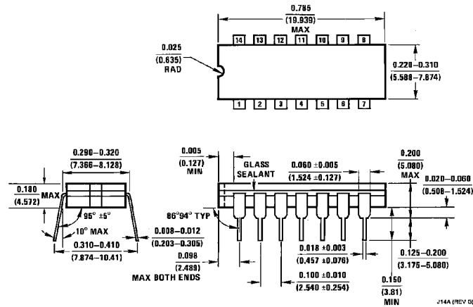
14-Lead Ceramic Dual-In-Line Package (J) Order Number 5420DMQB or DM5420J NS Package Number J14A
