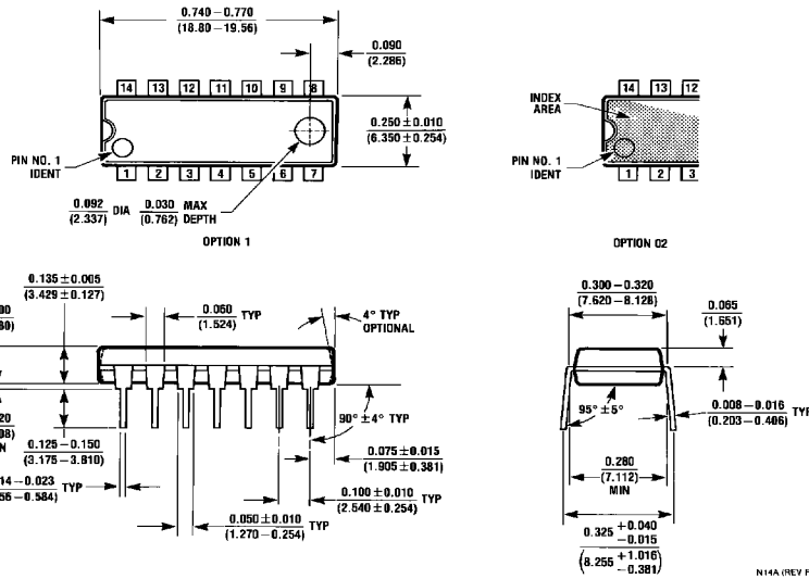
14-Lead Molded Dual-In-Line Package (N) Order Number DM7420N NS Package Number N14A
