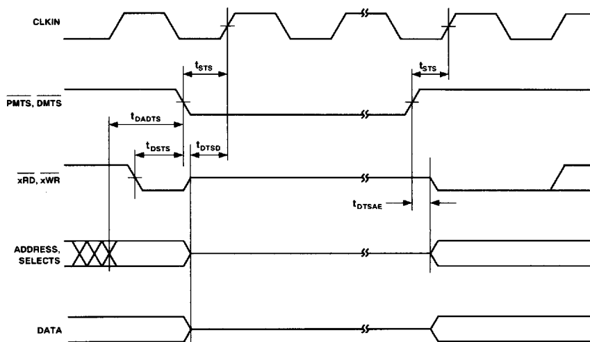
Figure 9. External Memory Three-State Control
