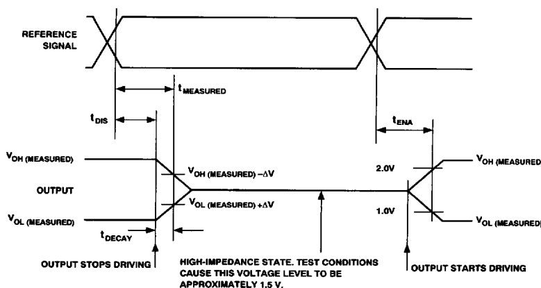
Figure 13. Output Enable/Disable
