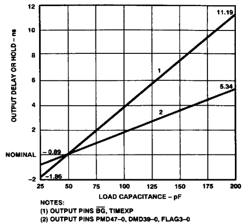
Figure 18. Typical Output Delay or Hold vs. Load Capacitance (at Maximum Case Temperature)
