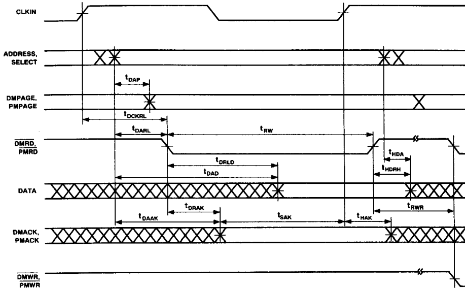
Figure 10. Memory Read
