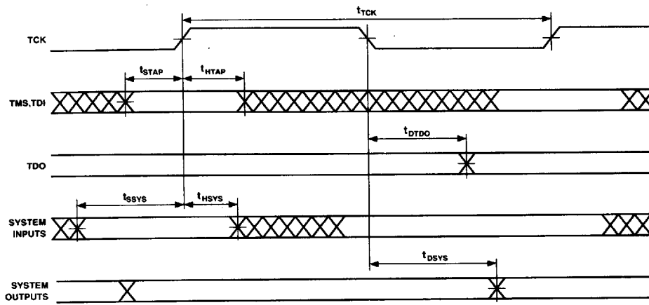
Figure 12. IEEE 1149.1 Test Access Port
