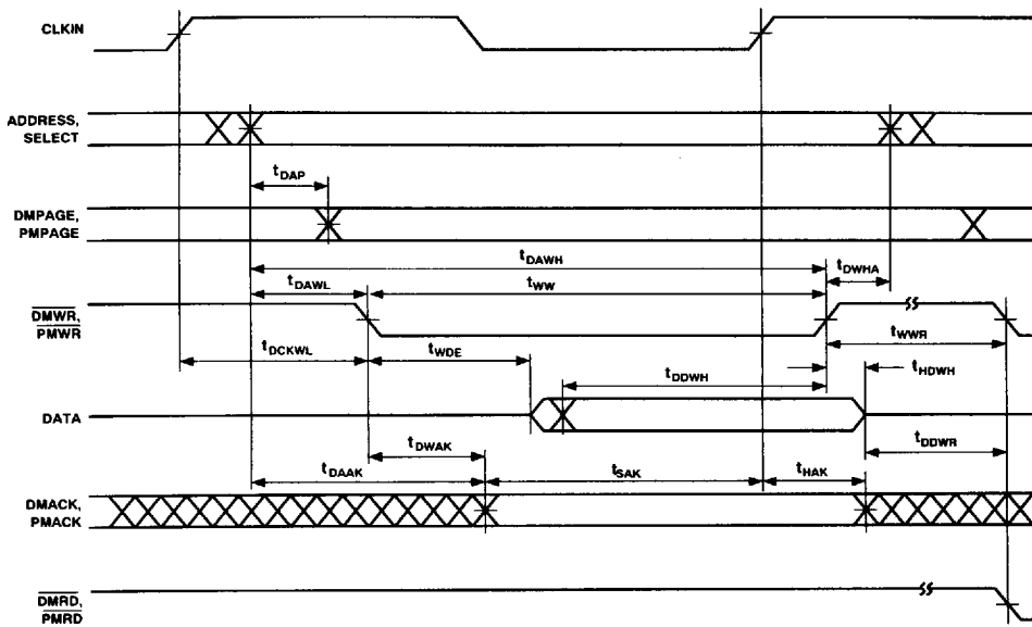
Figure 11. Memory Write
