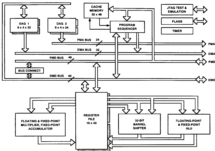
Figure 1. ADSP-21020 Block Diagram
