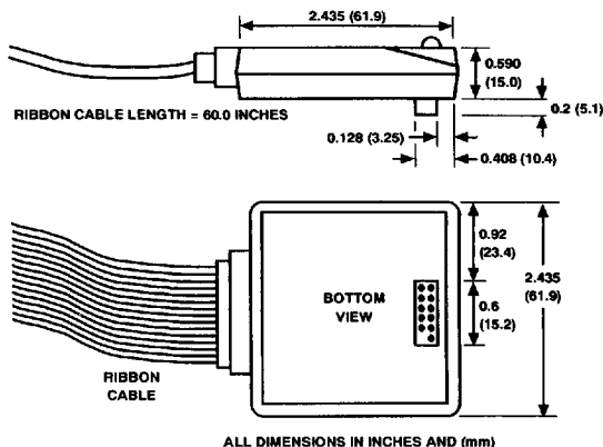
Figure 21. EZ-ICE Probe
