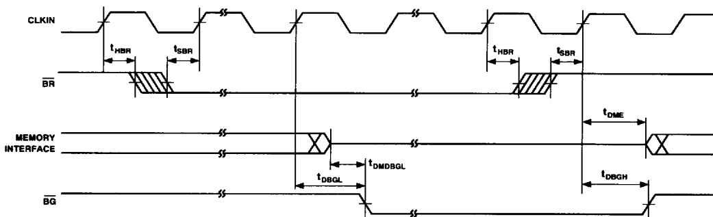
Figure 8. Bus Request/Bus Grant
