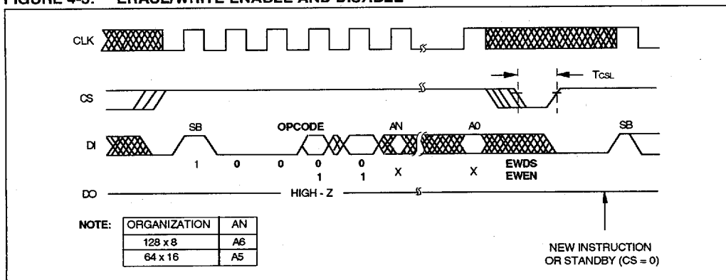
FIGURE 4-3: ERASE/WRITE ENABLE AND DISABLE
