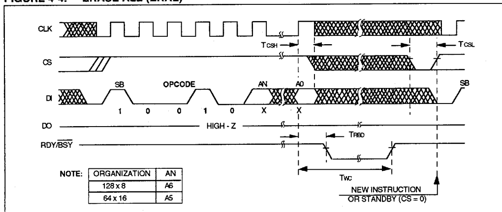
FIGURE 4-4: ERASE ALL (ERAL)
