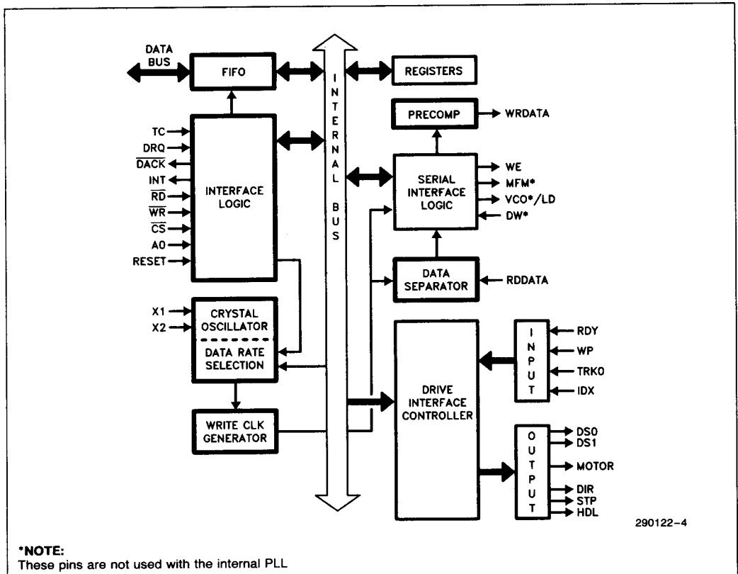
Figure 3. 82072 Block Diagram
