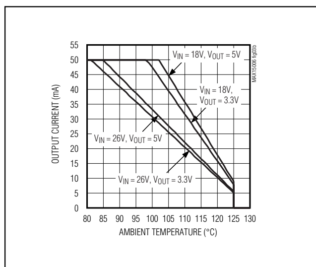
Figure 3b. Minimum Output Current vs. Ambient Temperature (8-Pin SO-EP)
