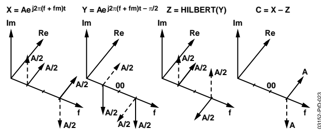
Figure 59. Negative Frequency Image Rejection
