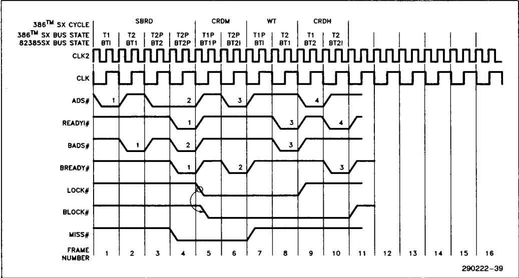
Figure 5-3K. LOCK # /BLOCK # in Non-Cacheable or Miss Cycles—(N = 1)
