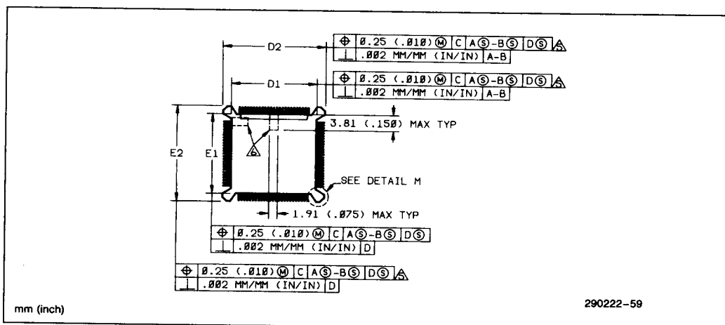
Figure 8-3.3. Molded Details
