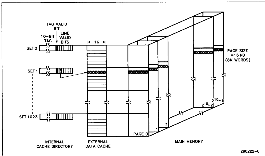
Figure 2-1. Direct Mapped Cache Organiztion
