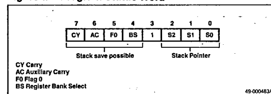
Figure 1. Program Status Word
