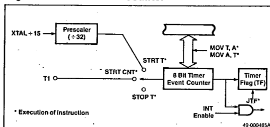
Figure 2. Timer/Event Counter
