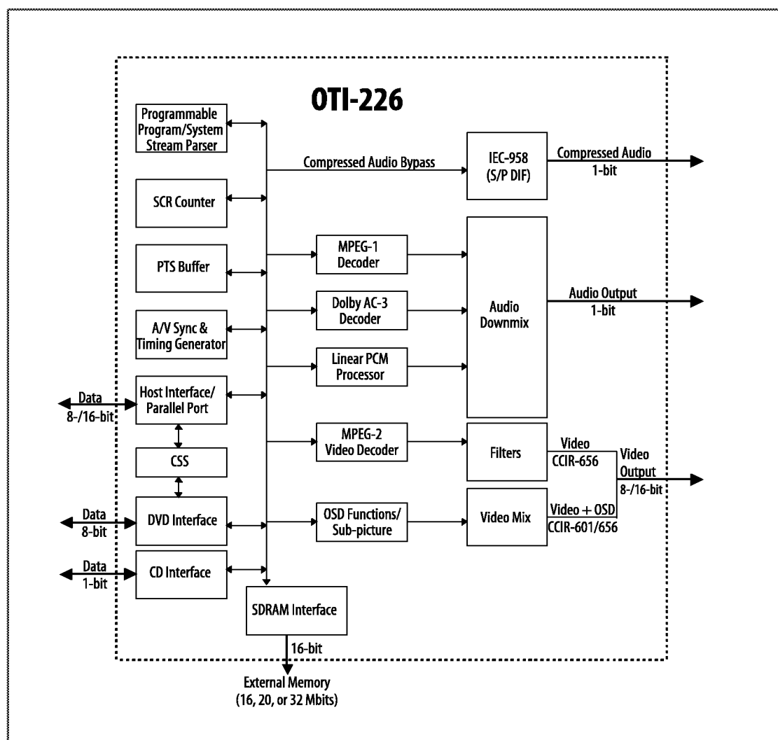
OTI-226 Architecture
