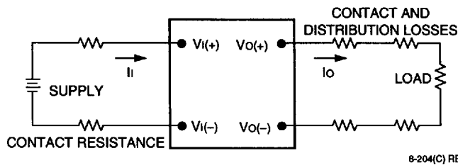
Figure 1. Input Reflected-Ripple Test Setup
