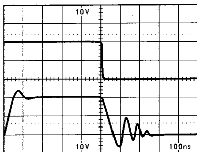
FIGURE 17. LH0032 Unity Gain Non-Inverting Large Signal Pulse Response: T_A = 25^\circ\text{C} , C_C = 10\text{ pF} , C_A = 100\text{ pF}
