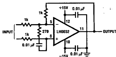
FIGURE 20. LH0032 Non-Compensated Unity Gain Compensation
