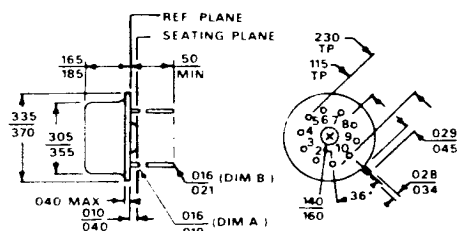
AD530H TO-100
