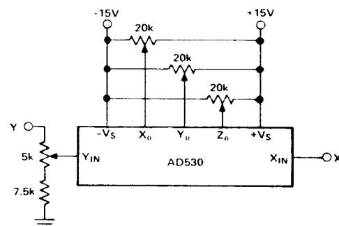
Figure 2. Adjustment Pot Connections (Multiplier Mode)
