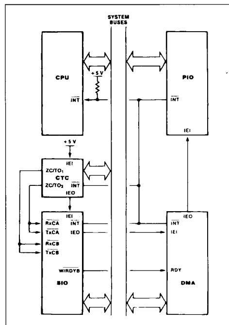
Figure 8 : A Typical Z80 Environment.
