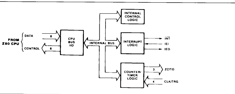
Figure 3 : Functional Block Diagram.
