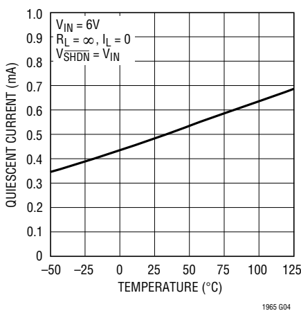
Quiescent Current
