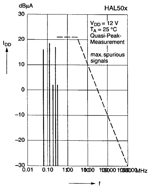
Spectrum of supply current
