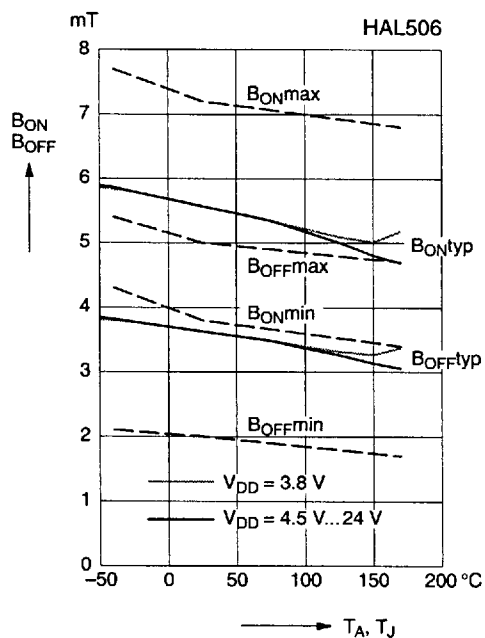
Magnetic switch points versus temperature
