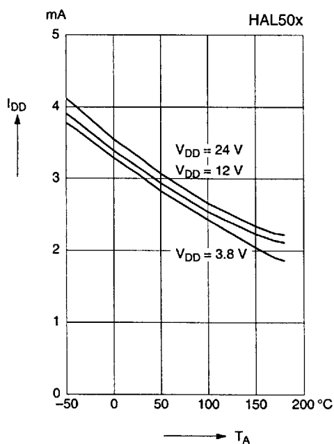
Supply current versus ambient temperature
