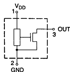
Fig. 1: Pin configuration
