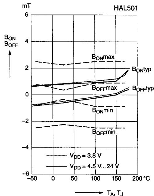
Magnetic switch points versus temperature
