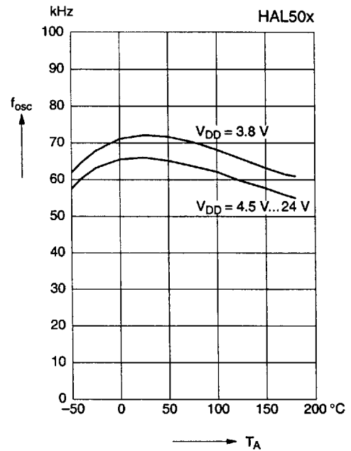
Internal chopper frequency versus ambient temperature
