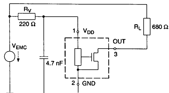
Fig. 9: Test circuit 1: test procedure for class C
