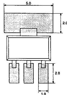
Fig. 7: Recommended pad size SOT-89A Dimensions in mm
