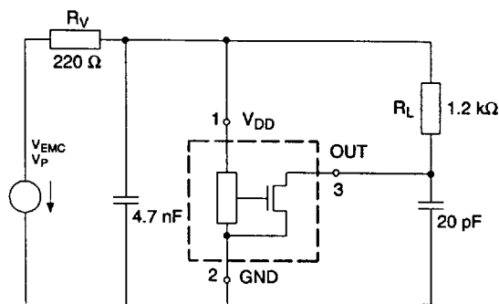
Fig. 8: Test circuit 2: test procedure for class A
