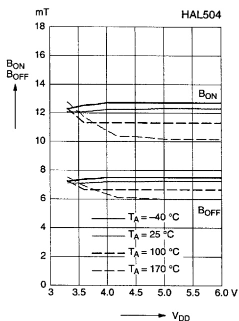
Magnetic switch points versus supply voltage
