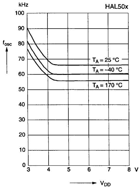
Internal chopper frequency versus supply voltage
