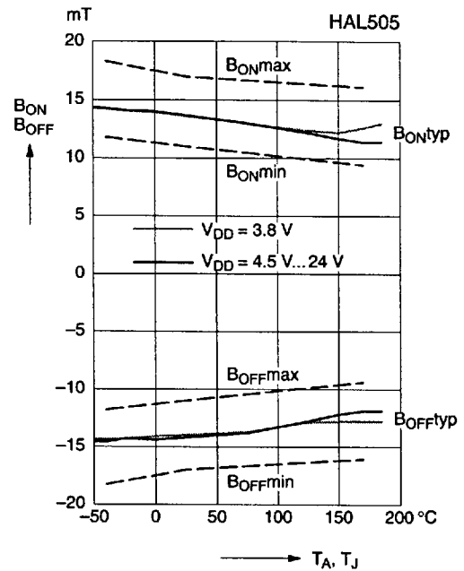
Magnetic switch points versus temperature
