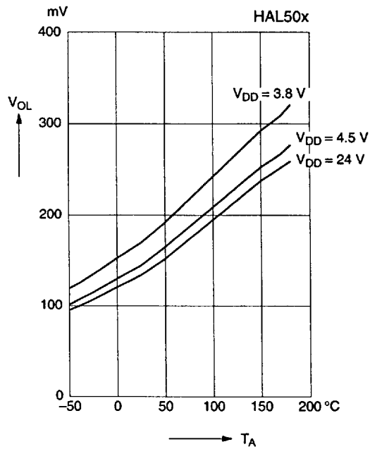
Output low voltage versus ambient temperature
