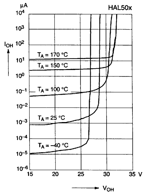
Output high current versus output voltage
