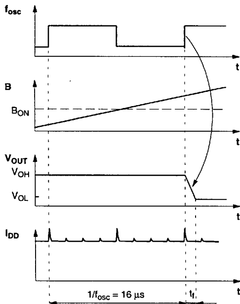
Fig. 3: Timing diagram
