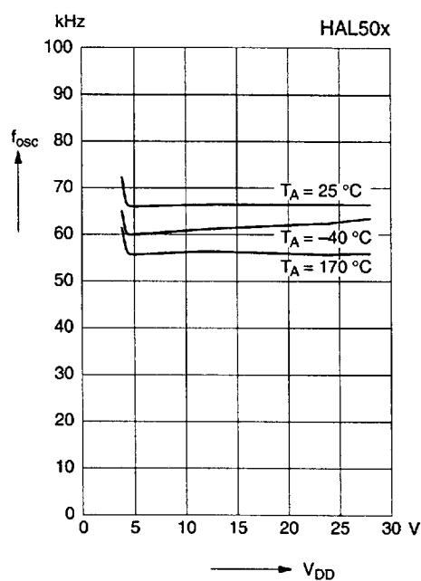
Internal chopper frequency versus supply voltage
