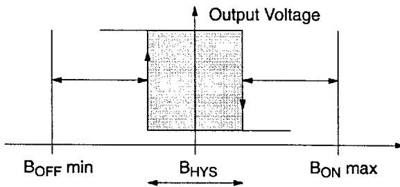
Fig. 6: Definition of magnetic switching points and hysteresis
