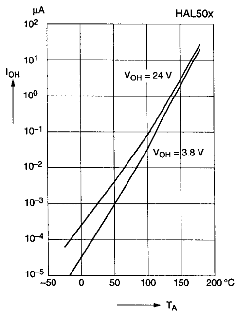
Output leakage current versus ambient temperature
