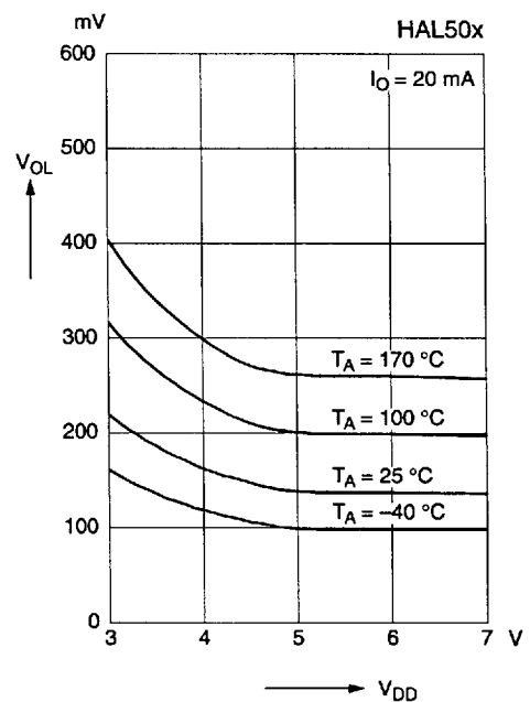
Output low voltage versus supply voltage
