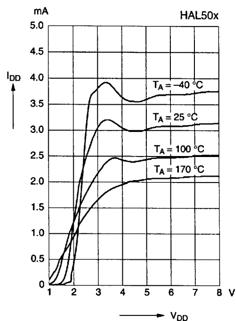
Supply current versus supply voltage
