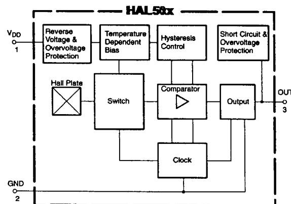
Fig. 2: HAL50x block diagram
