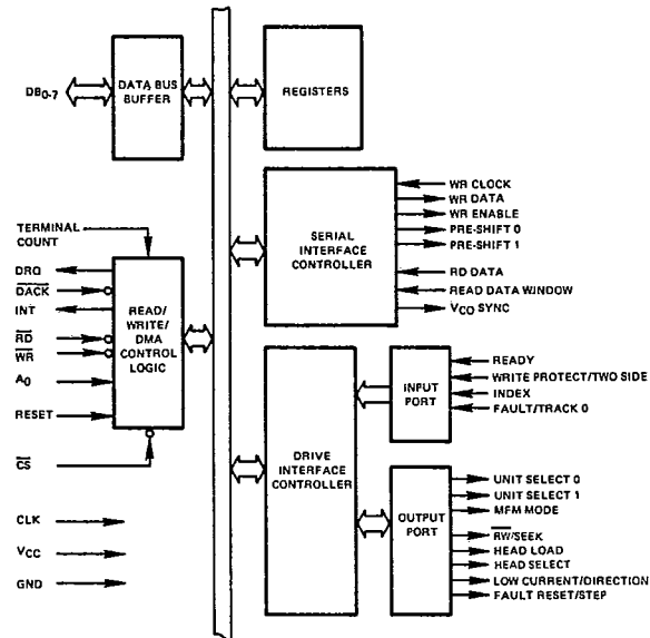
BLOCK DIAGRAM
