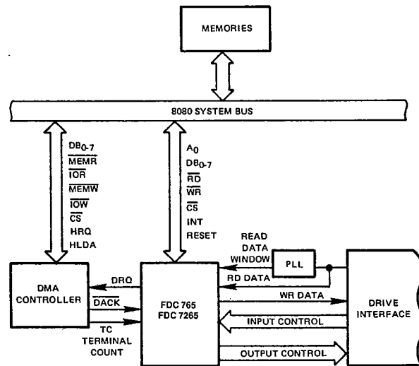
SYSTEM CONFIGURATION
