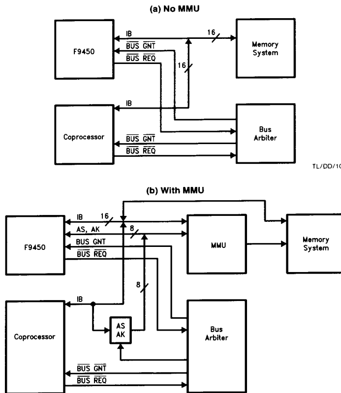
FIGURE 23. F9450/ Coprocessor Configuration
