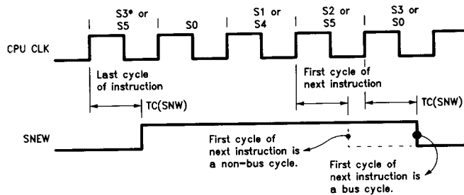
FIGURE 15. SNEW Discrete Timing Diagram
