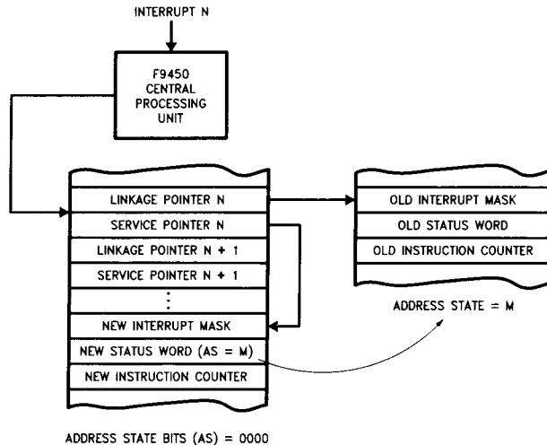
FIGURE 3. Interrupt Vectors
