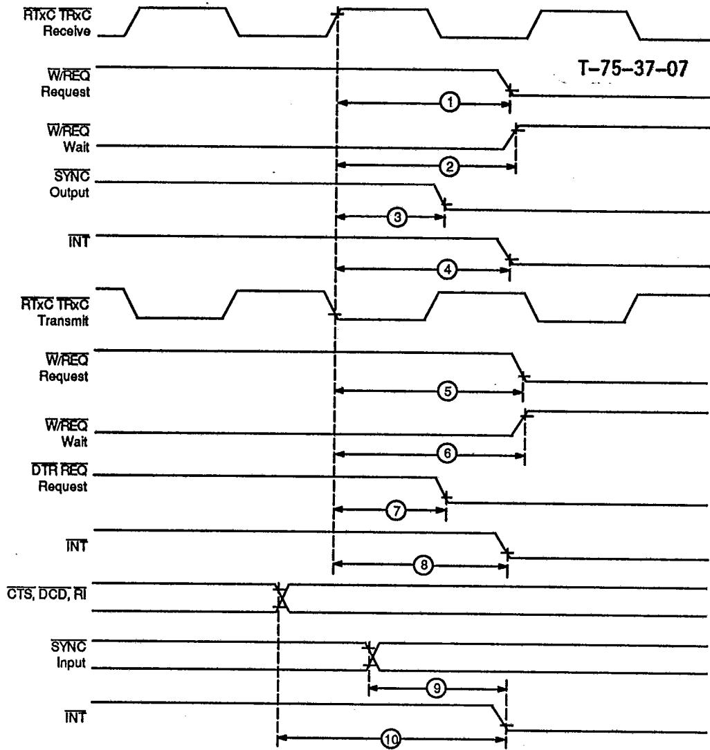
Figure 20. System Timing
