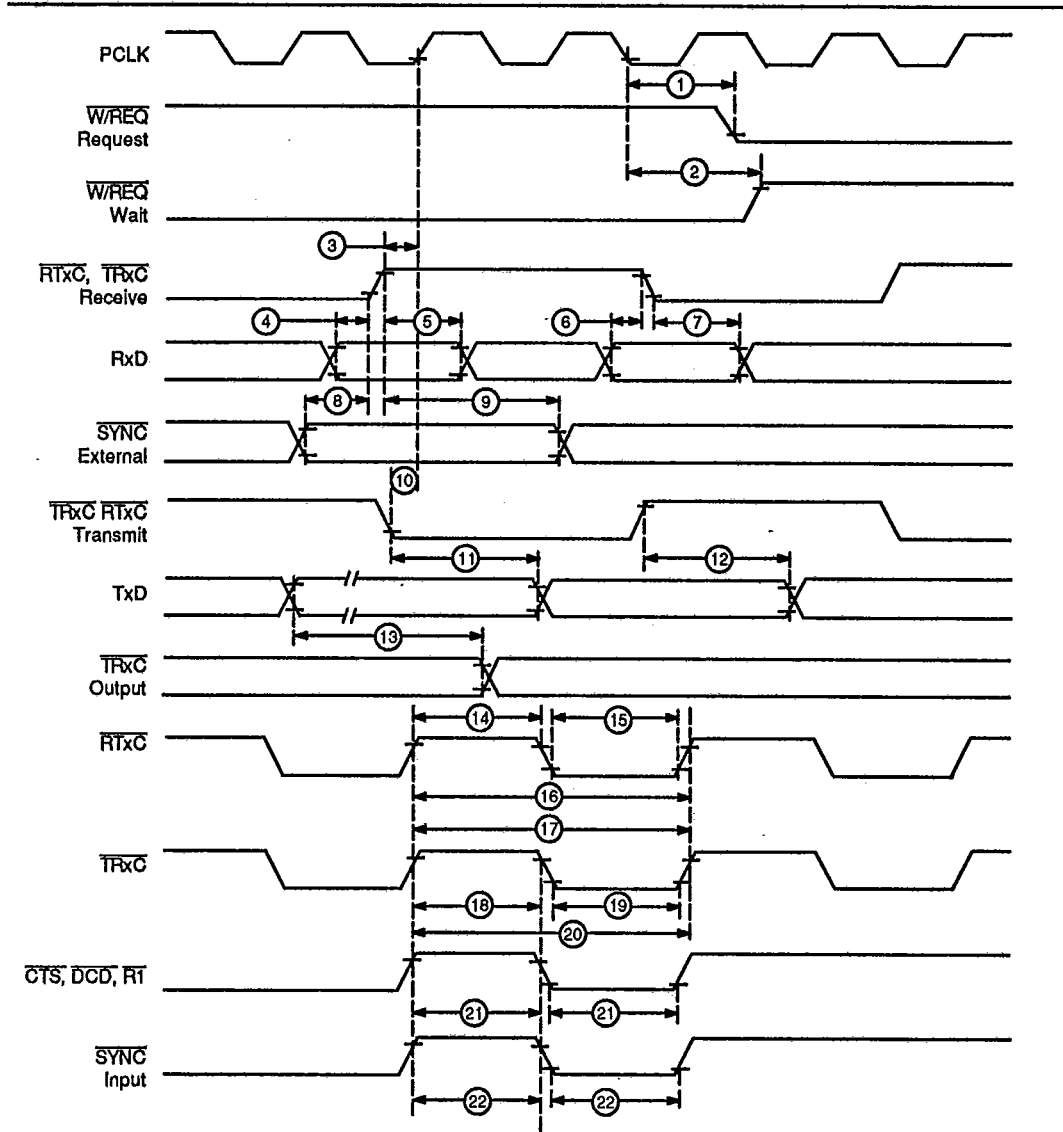
Figure 19. General Timing
