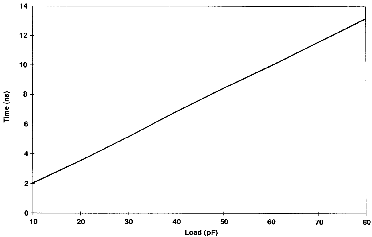
Figure 17. 3.3-V I/O Drive Type C Rise Time
