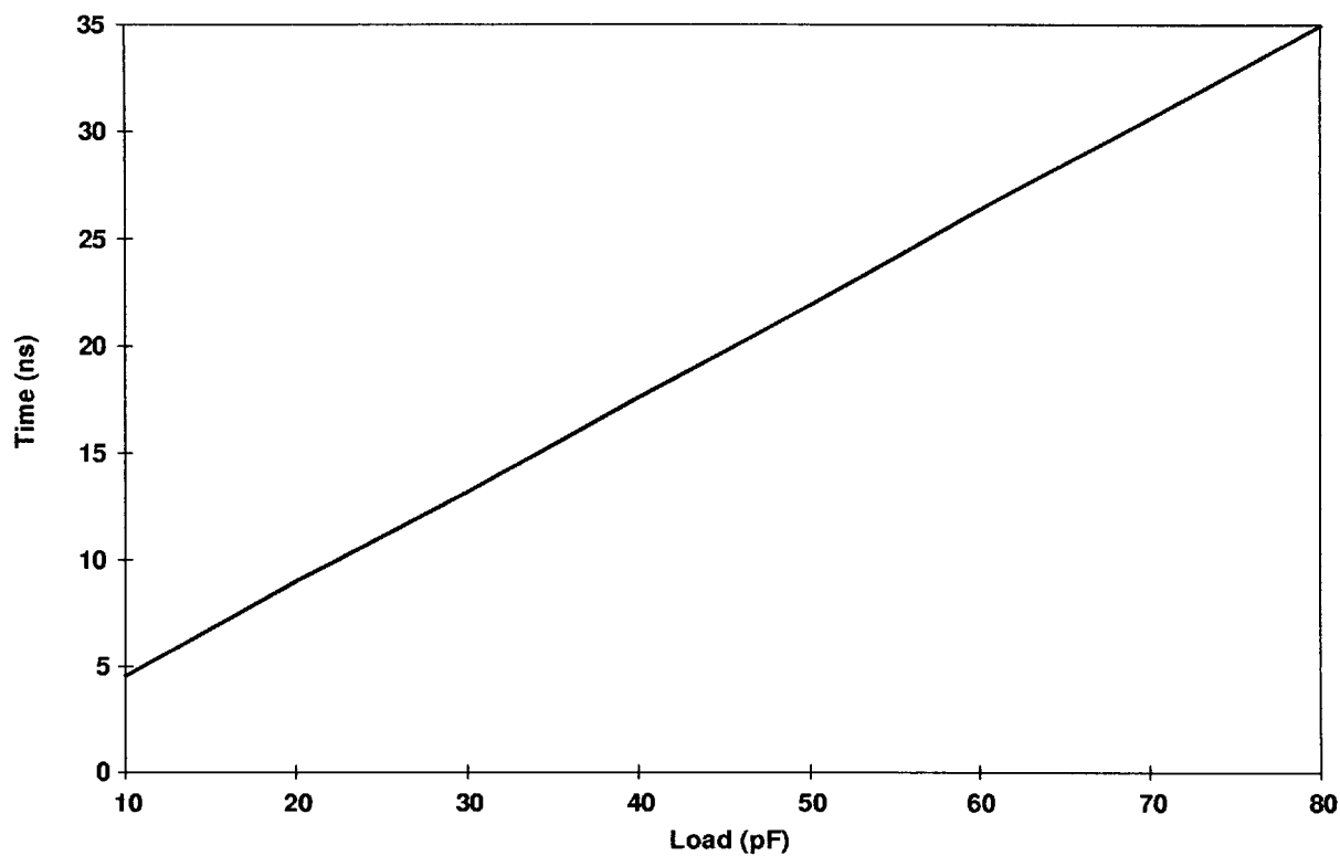
Figure 26. 3.3-V I/O Drive Type A Fall Time
