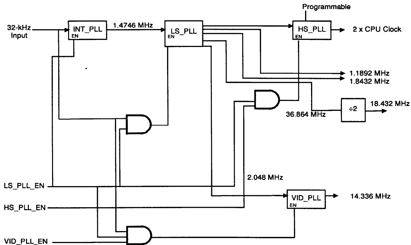
Figure 1. PLL Block Diagram
