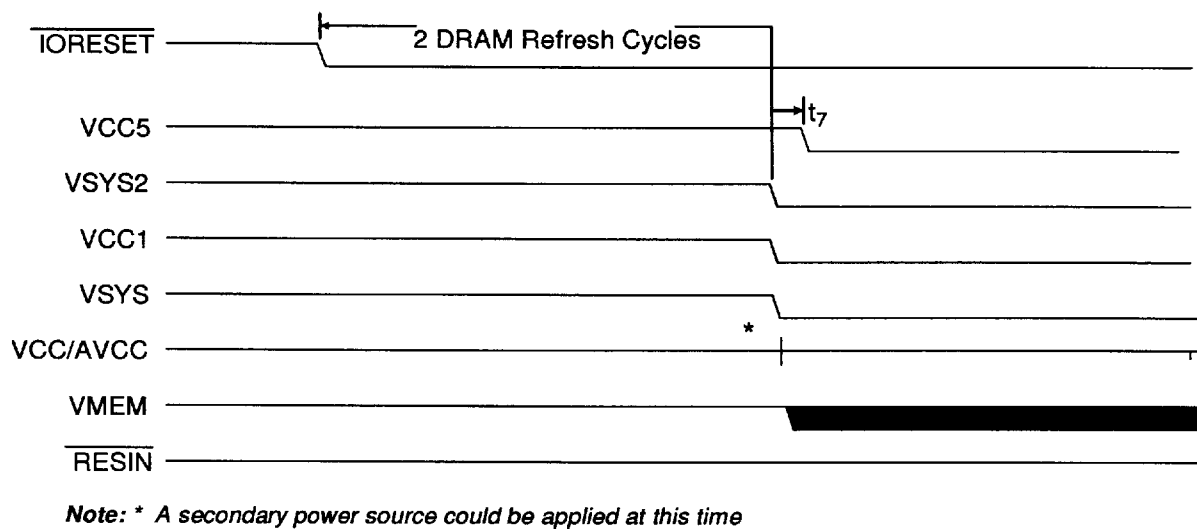
Figure 34. Entering Micro Power Off Mode (DRAM Refresh Enabled)
