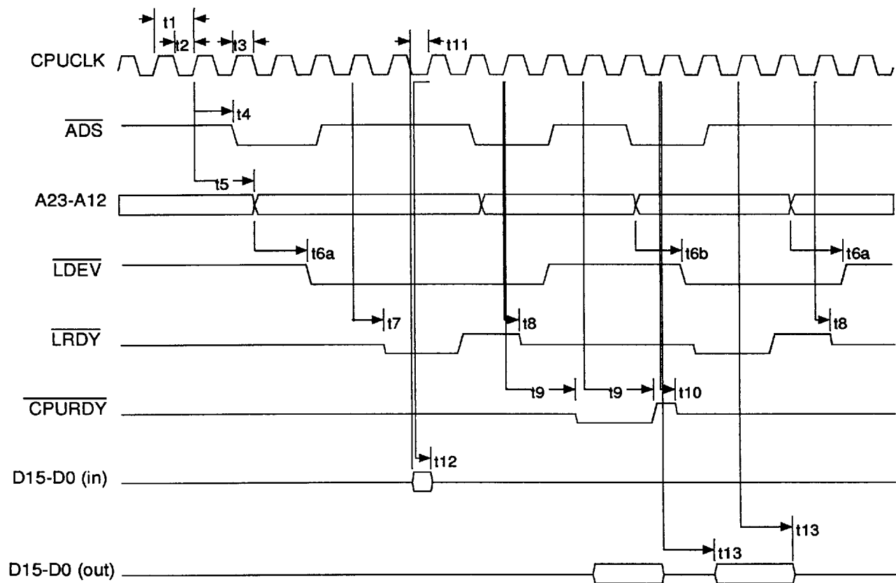
Figure 38. Local Bus Interface
