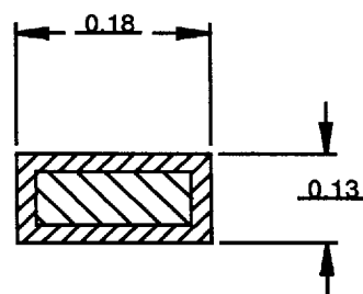
Section S-S
