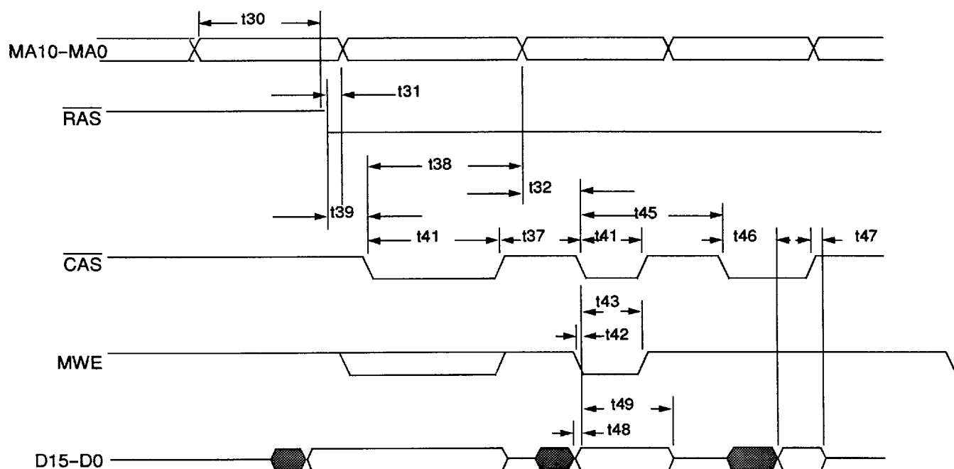
Figure 35. DRAM Timings, Page Hit
