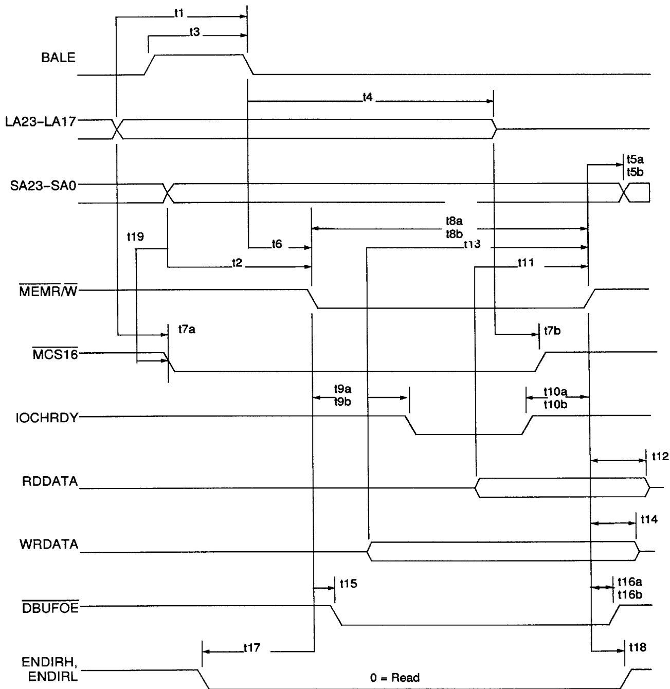
Figure 49. ISA Memory Read/Write 16-Bit Cycle
