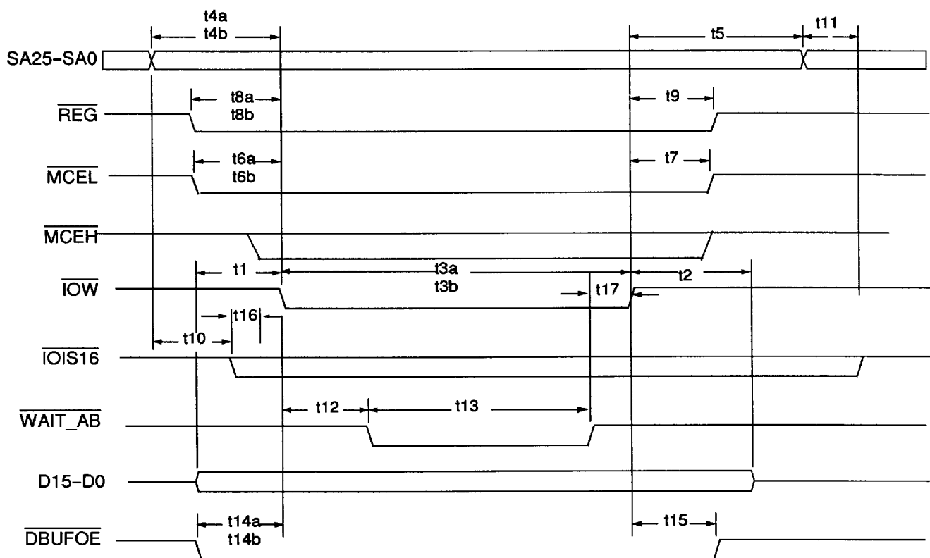
Figure 44. PCMCIA I/O Write Cycle
