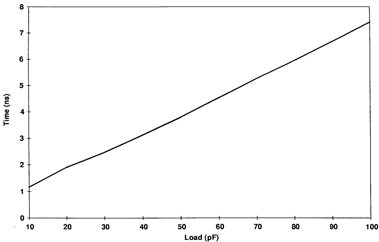
Figure 11. 5-V I/O Drive Type E Rise Time
