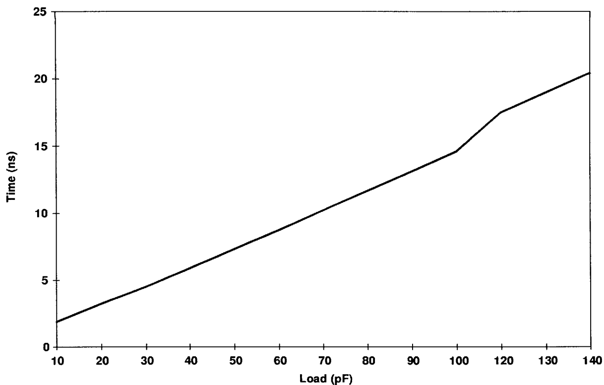
Figure 14. 3.3-V I/O Drive Type D Fall Time
