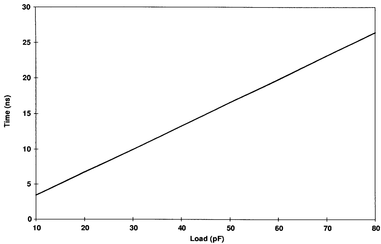
Figure 28. 5-V I/O Drive Type A Fall Time
