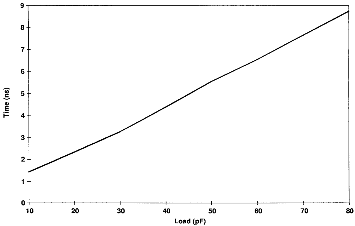
Figure 20. 5-V I/O Drive Type C Fall Time
