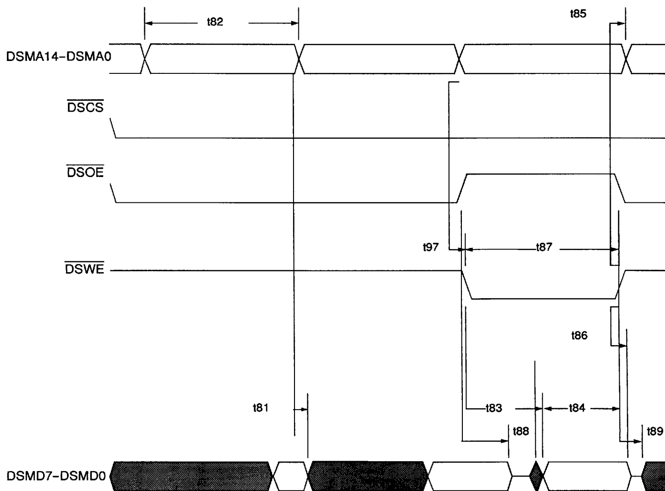
Figure 39. Display SRAM Timings
