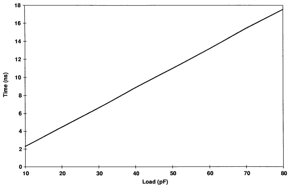
Figure 22. 3.3-V I/O Drive Type B Fall Time
