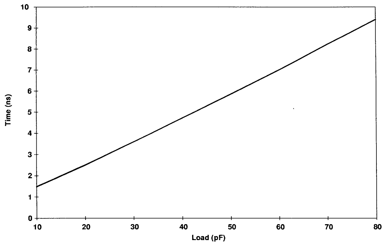
Figure 19. 5-V I/O Drive Type C Rise Time
