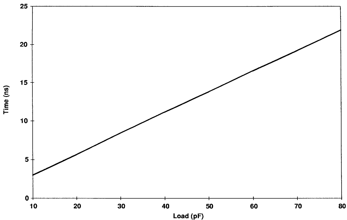
Figure 21. 3.3-V I/O Drive B Rise Time
