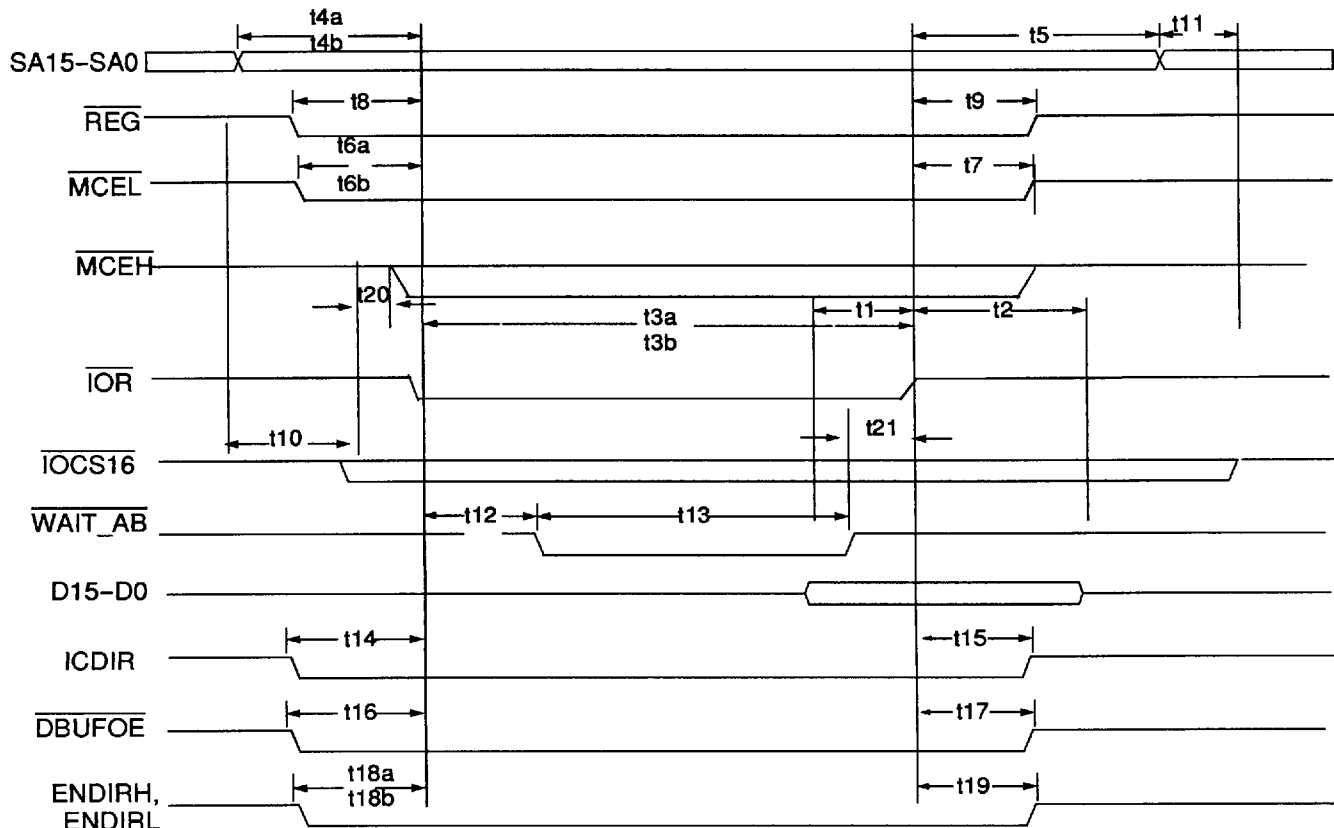
Figure 43. PCMCIA I/O Read Cycle
