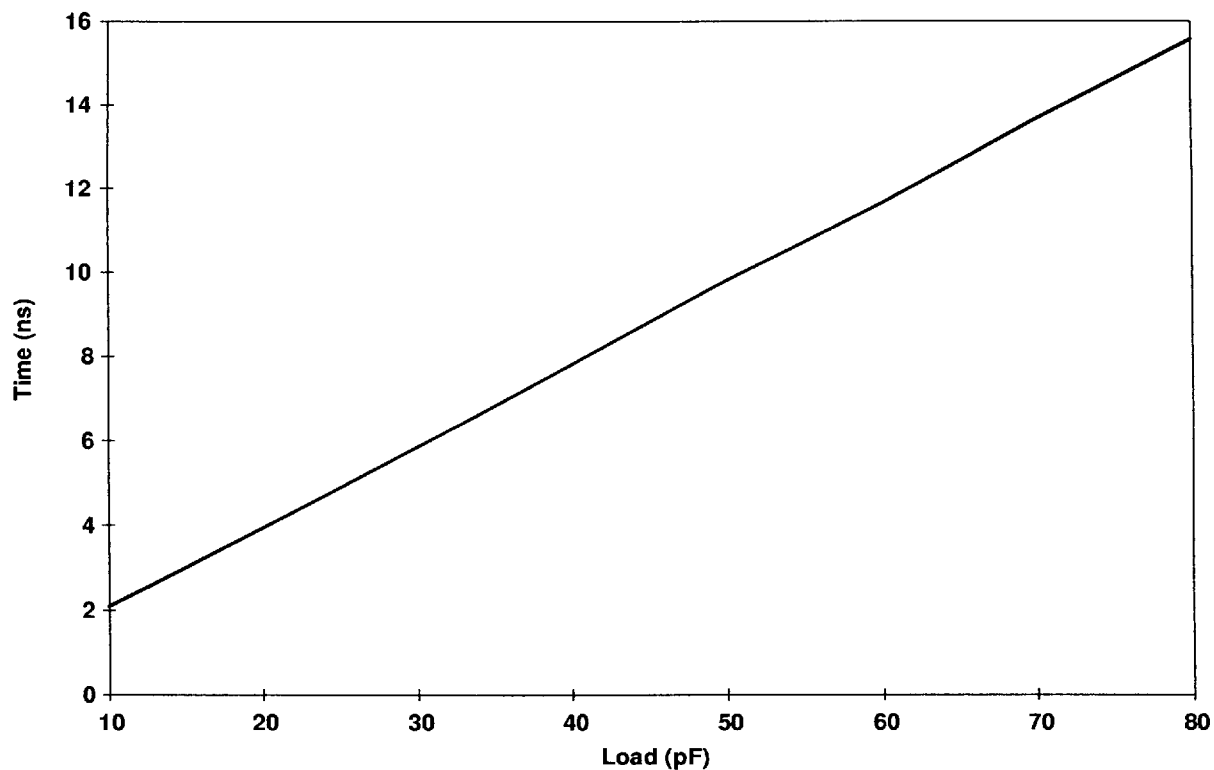
Figure 23. 5-V I/O Drive Type B Rise Time
