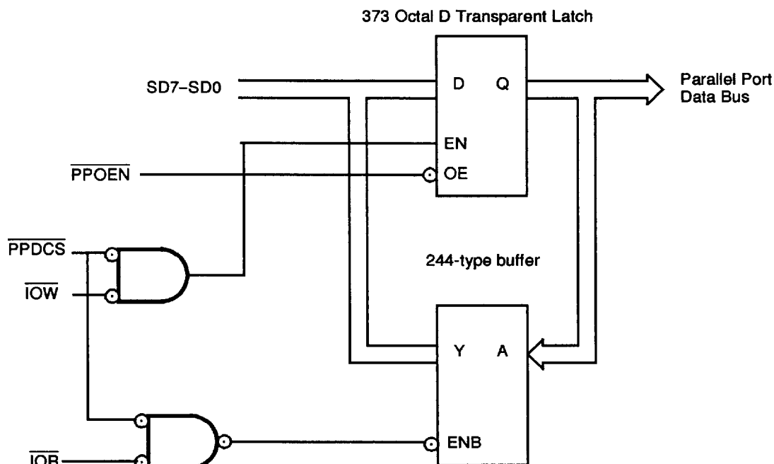
Figure 6. Am386SC300 CPU Bidirectional Parallel Port and EPP Implementation
