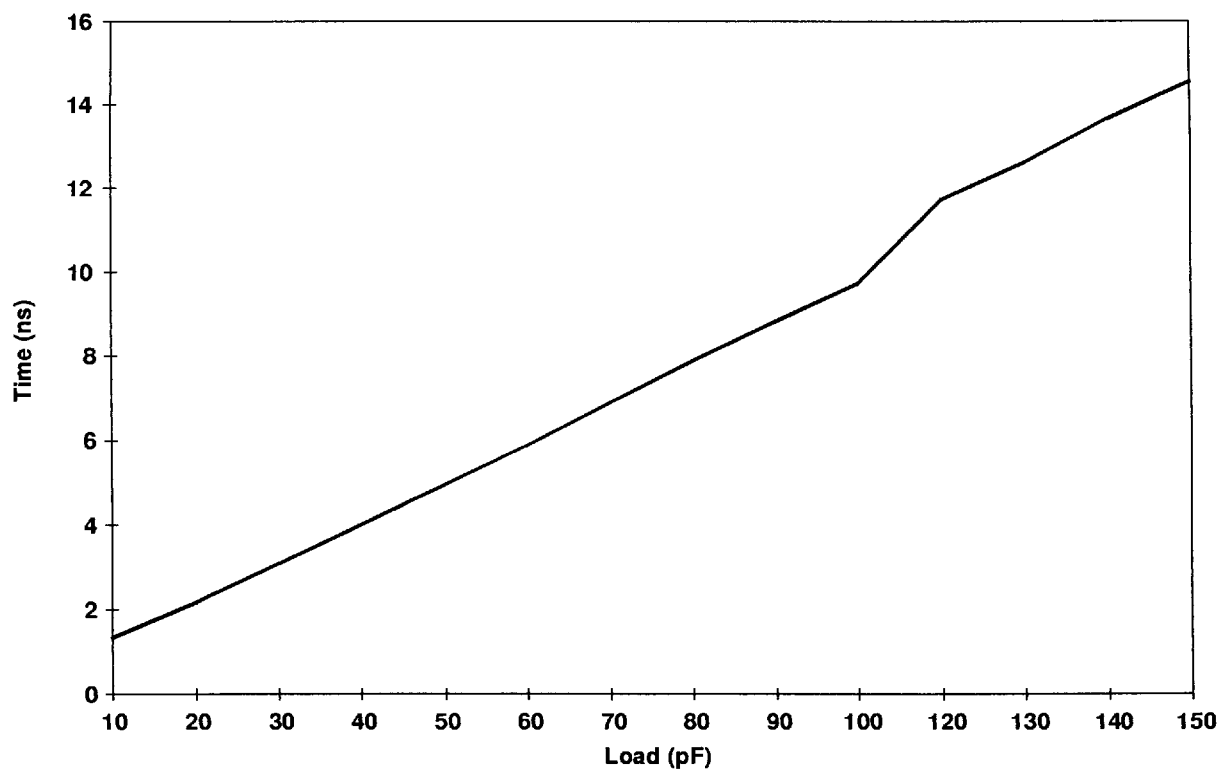
Figure 15. 5-V I/O Drive Type D Rise Time
