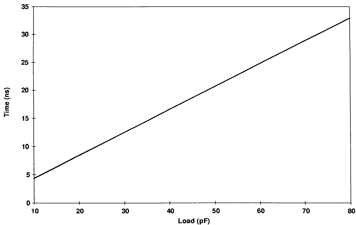
Figure 25. 3.3-V I/O Drive Type A Rise Time
