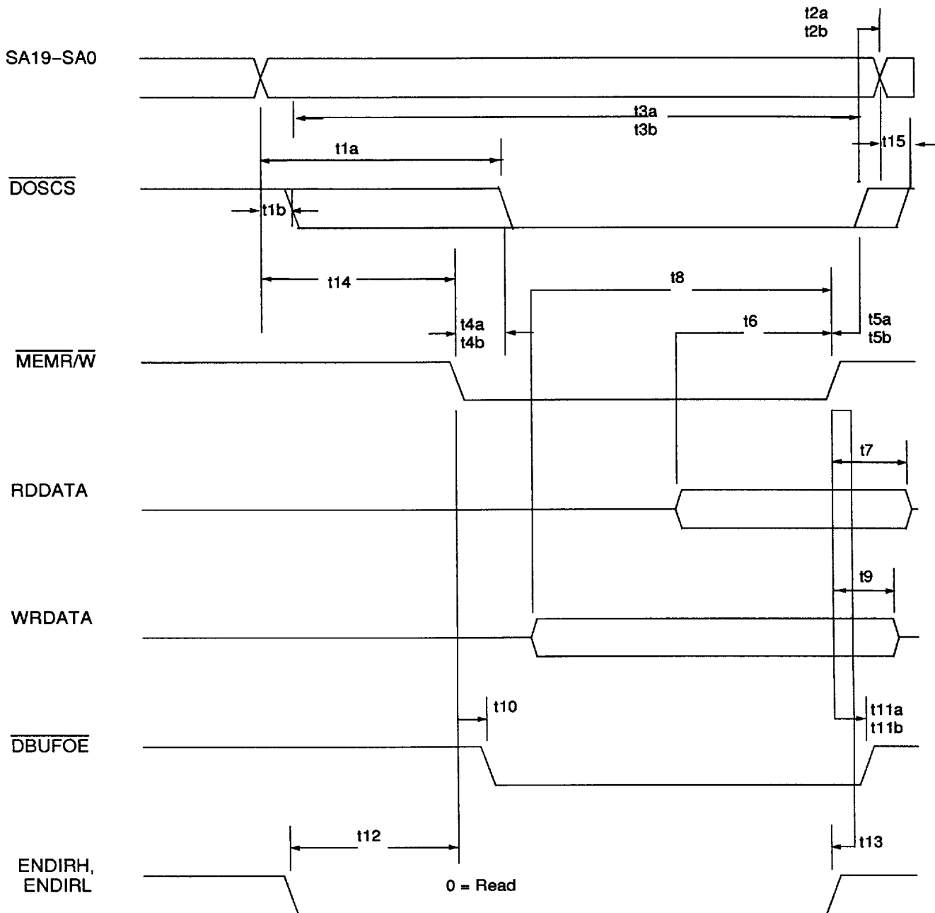
Figure 46. DOS ROM Read/Write 8-Bit Cycle
