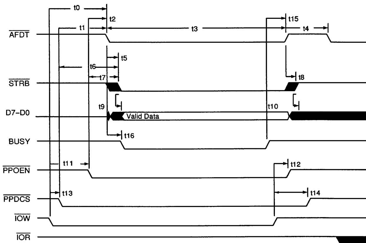
Figure 53. EPP Data Register Write Cycle
