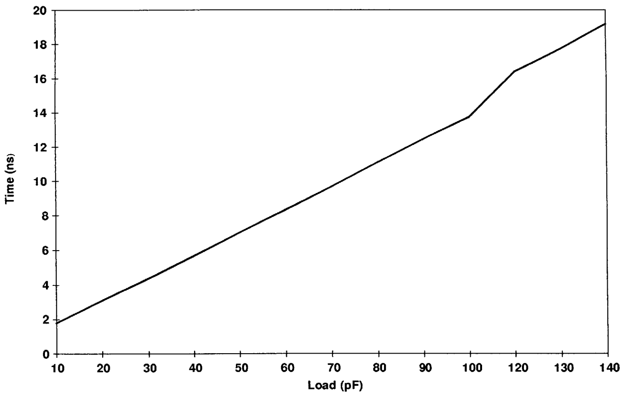
Figure 13. 3.3-V I/O Drive Type D Rise Time
