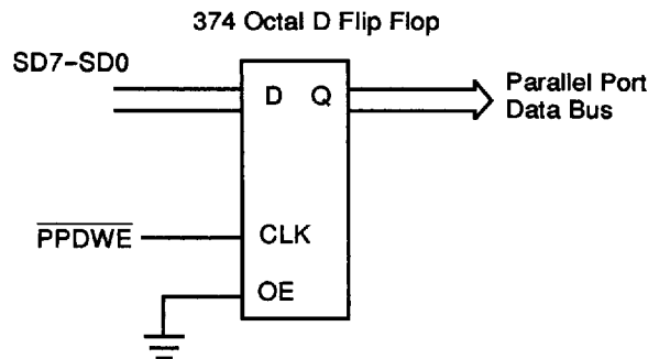
Figure 5. Am386SC300 CPU Unidirectional Parallel Port Data Bus Implementation
