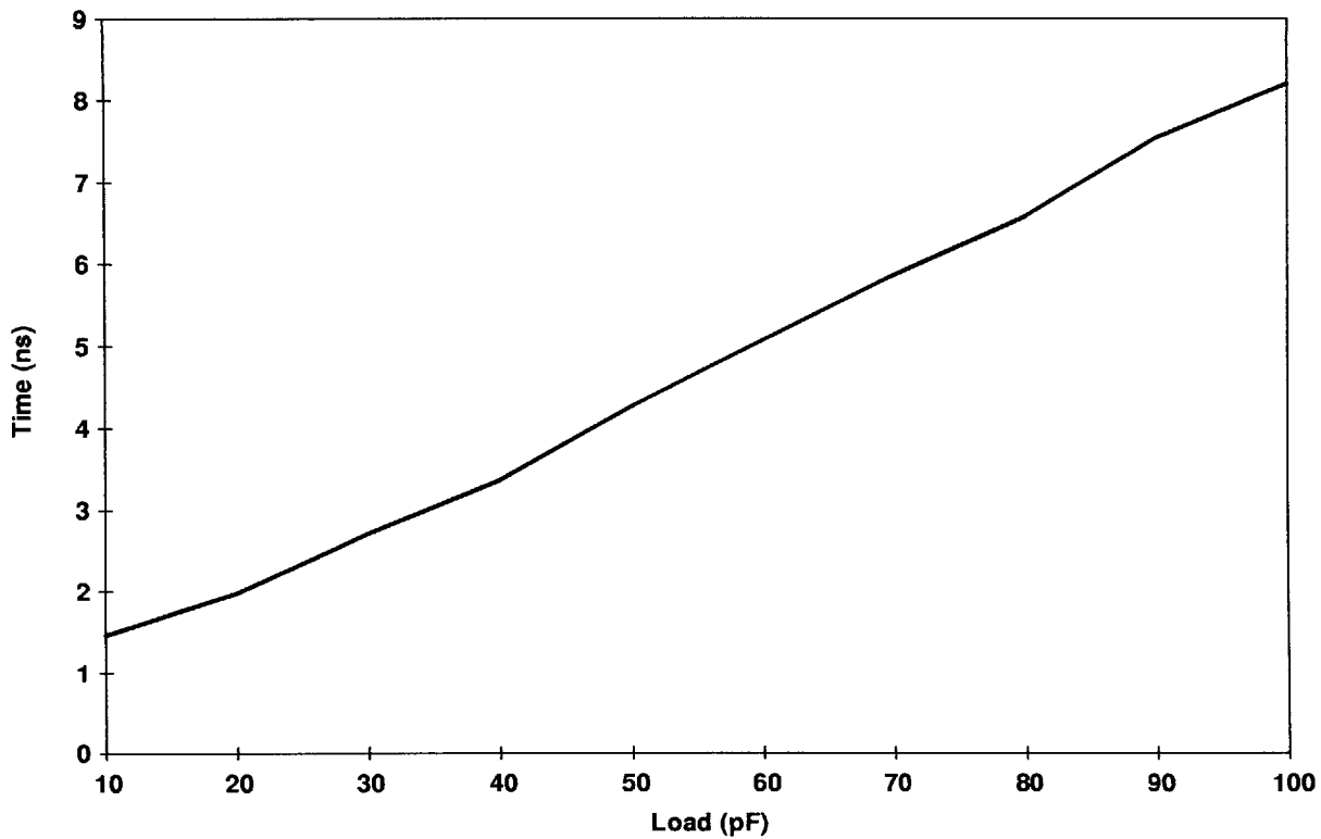
Figure 12. 5-V I/O Drive Type E Fall Time
