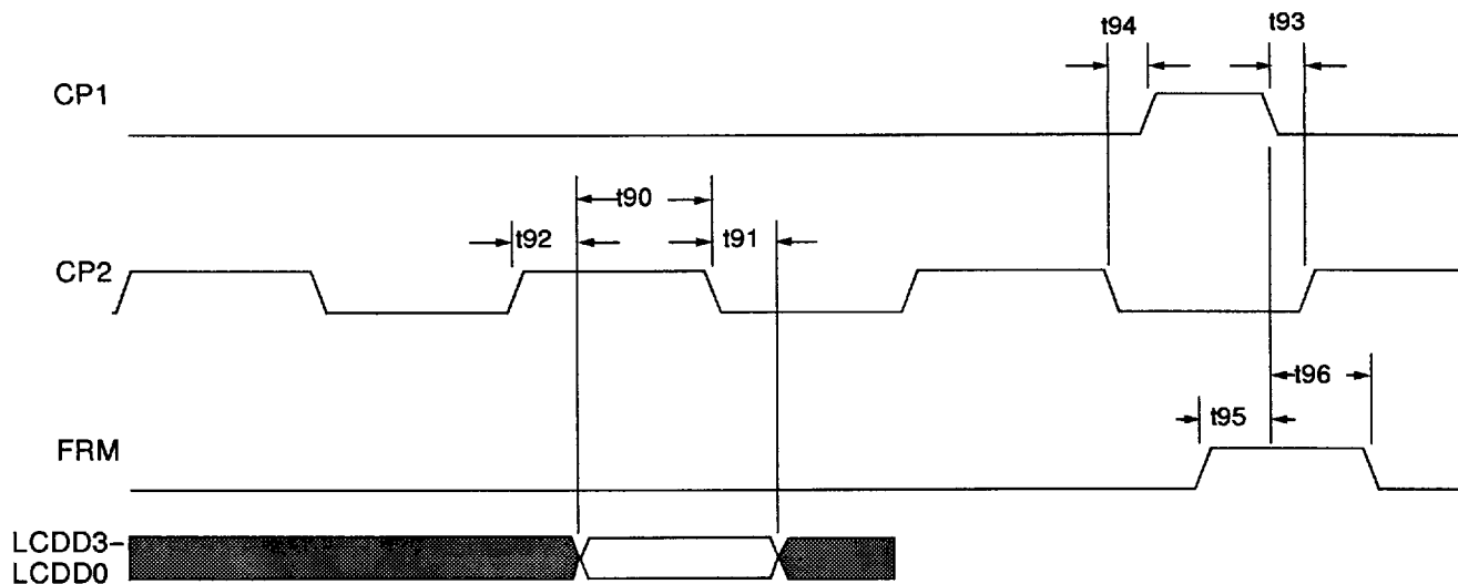
Figure 40. LCD Interface Timings
