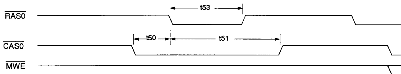
Figure 37. DRAM Timings, Refresh Cycle
