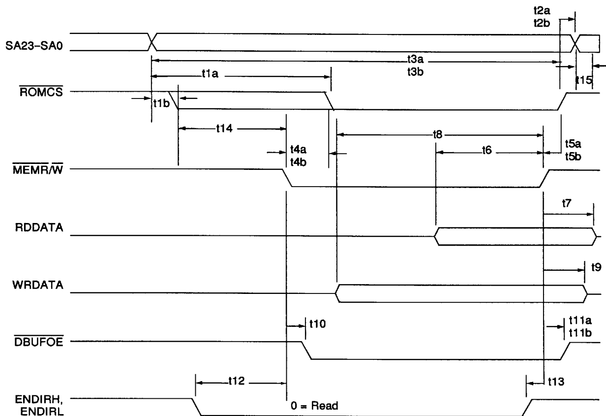
Figure 45. BIOS ROM Read/Write 8-Bit Cycle
