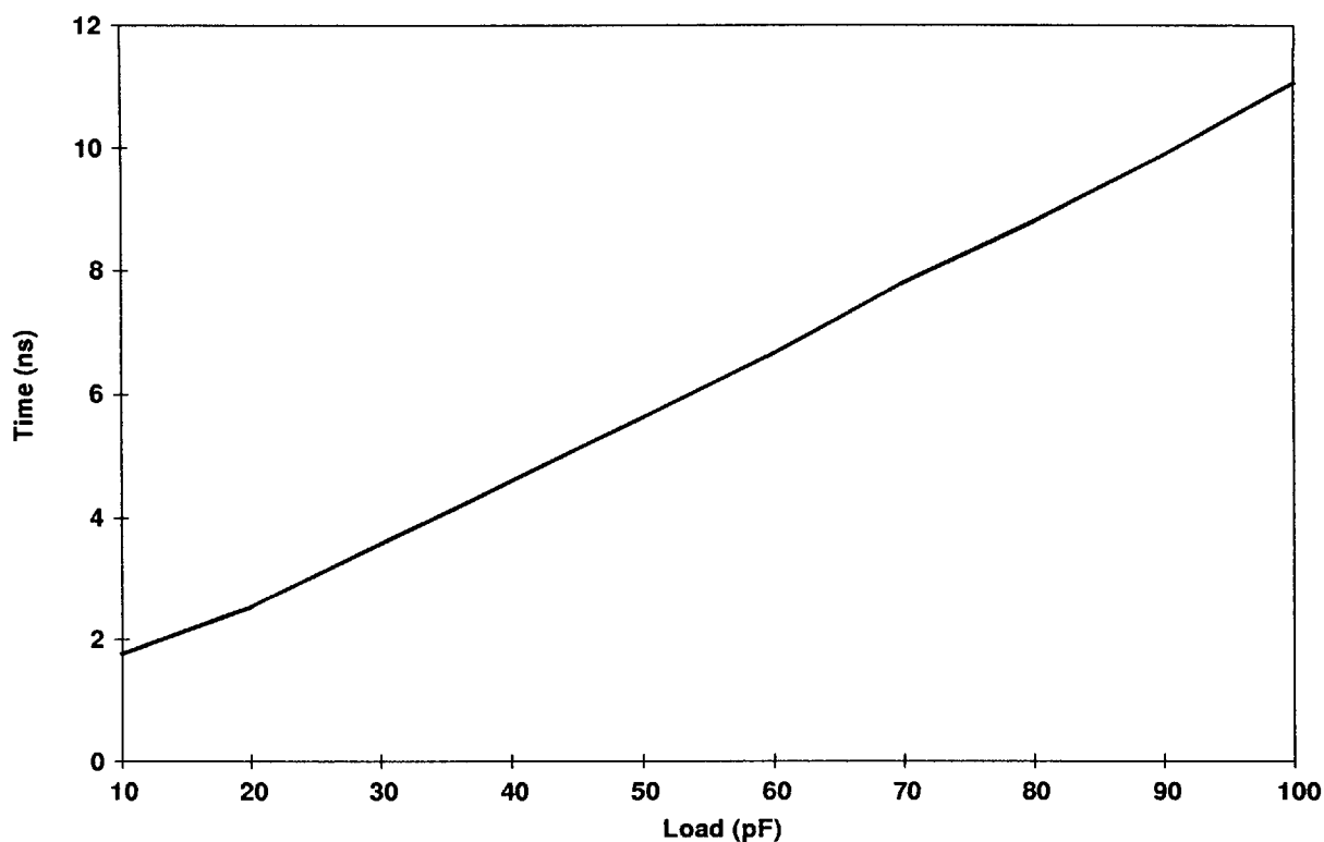
Figure 10. 3.3-V I/O Drive Type E Fall Time
