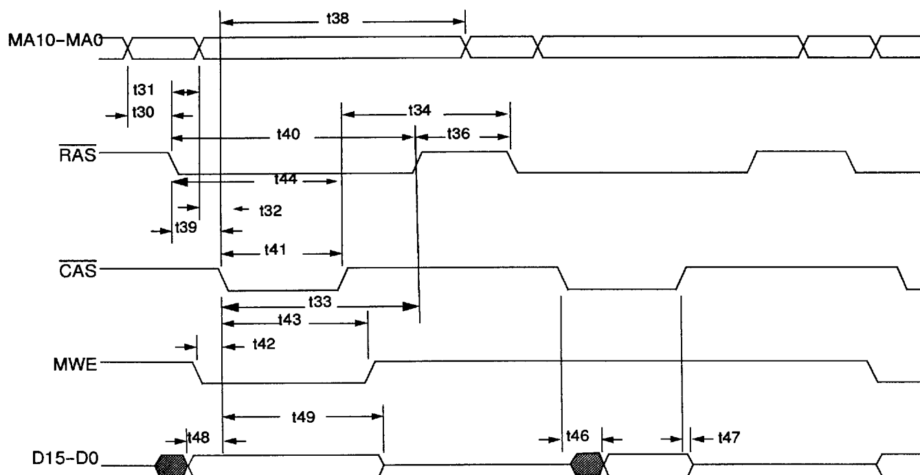
Figure 36. DRAM Timings, Page Miss
