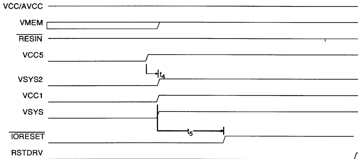
Figure 32. Micro Power Off Mode Exit
