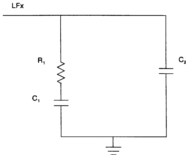
Figure 30. Loop-Filter Component
