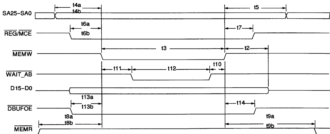
Figure 42. PCMCIA Memory Write Cycle
