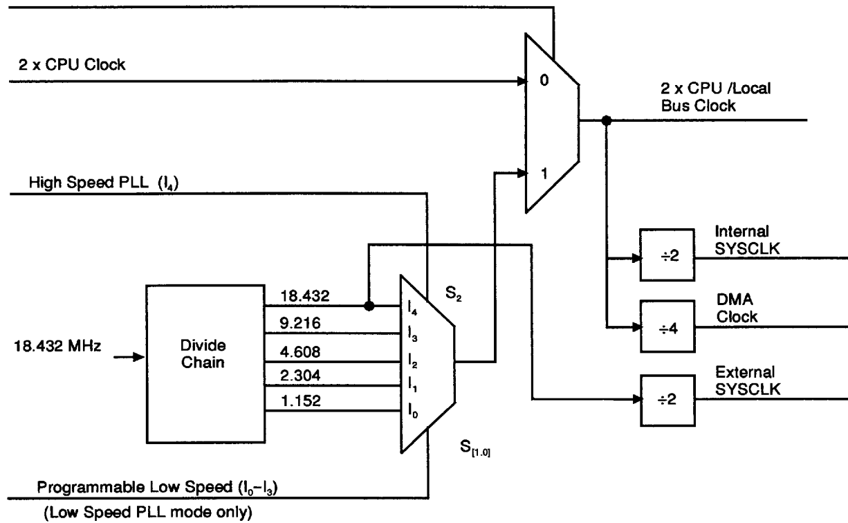
Figure 2. Clock Steering Block Diagram
