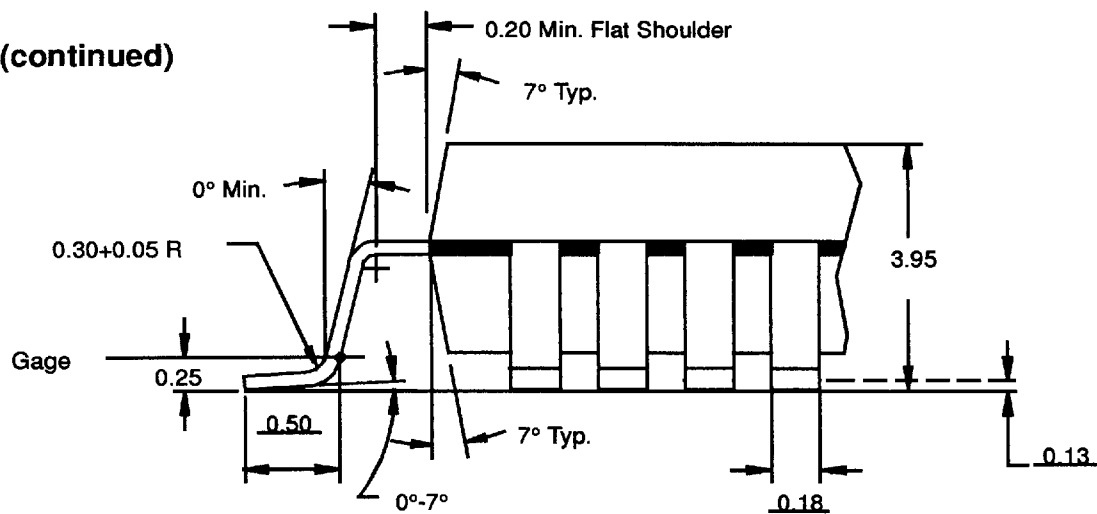
Detail X
