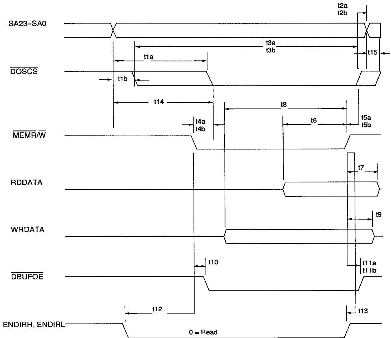
Figure 47. DOS ROM Read/Write 16-Bit Cycle
