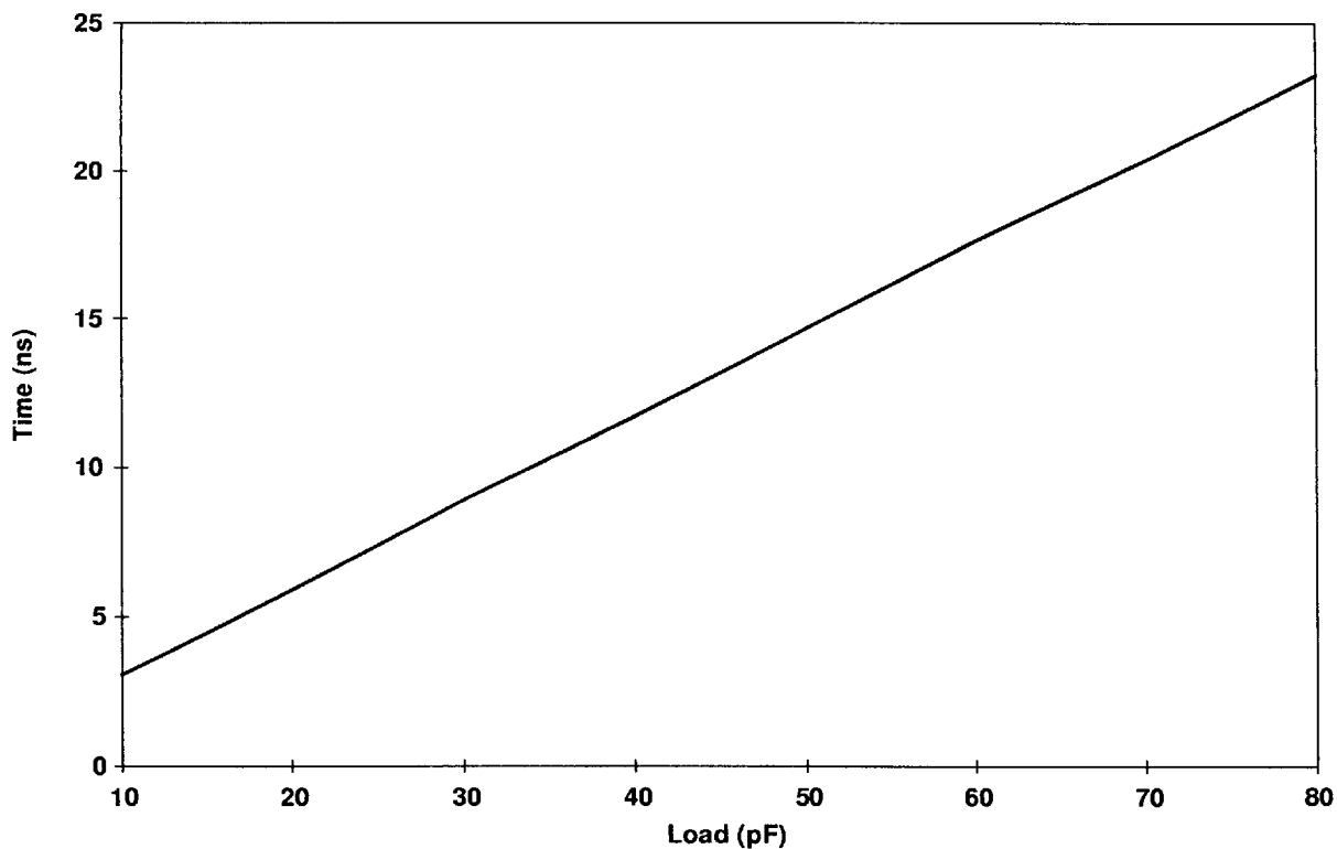
Figure 27. 5-V I/O Drive Type A Rise Time
