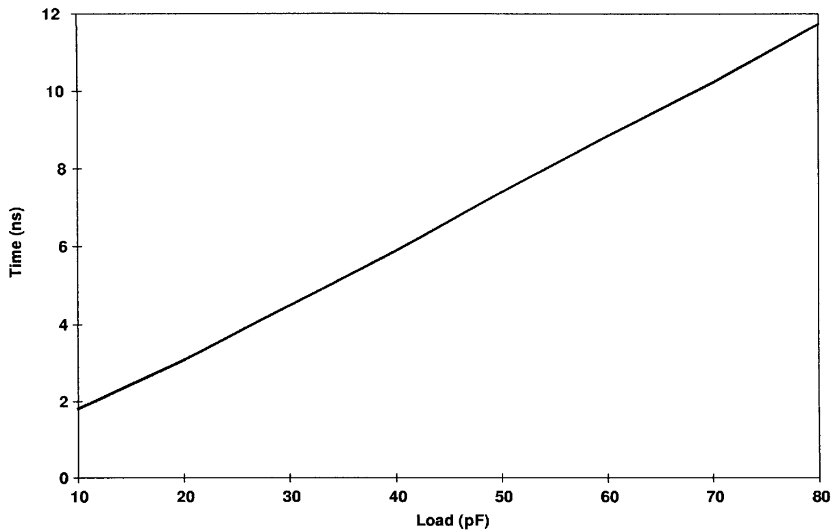
Figure 18. 3.3-V I/O Drive Type C Fall Time
