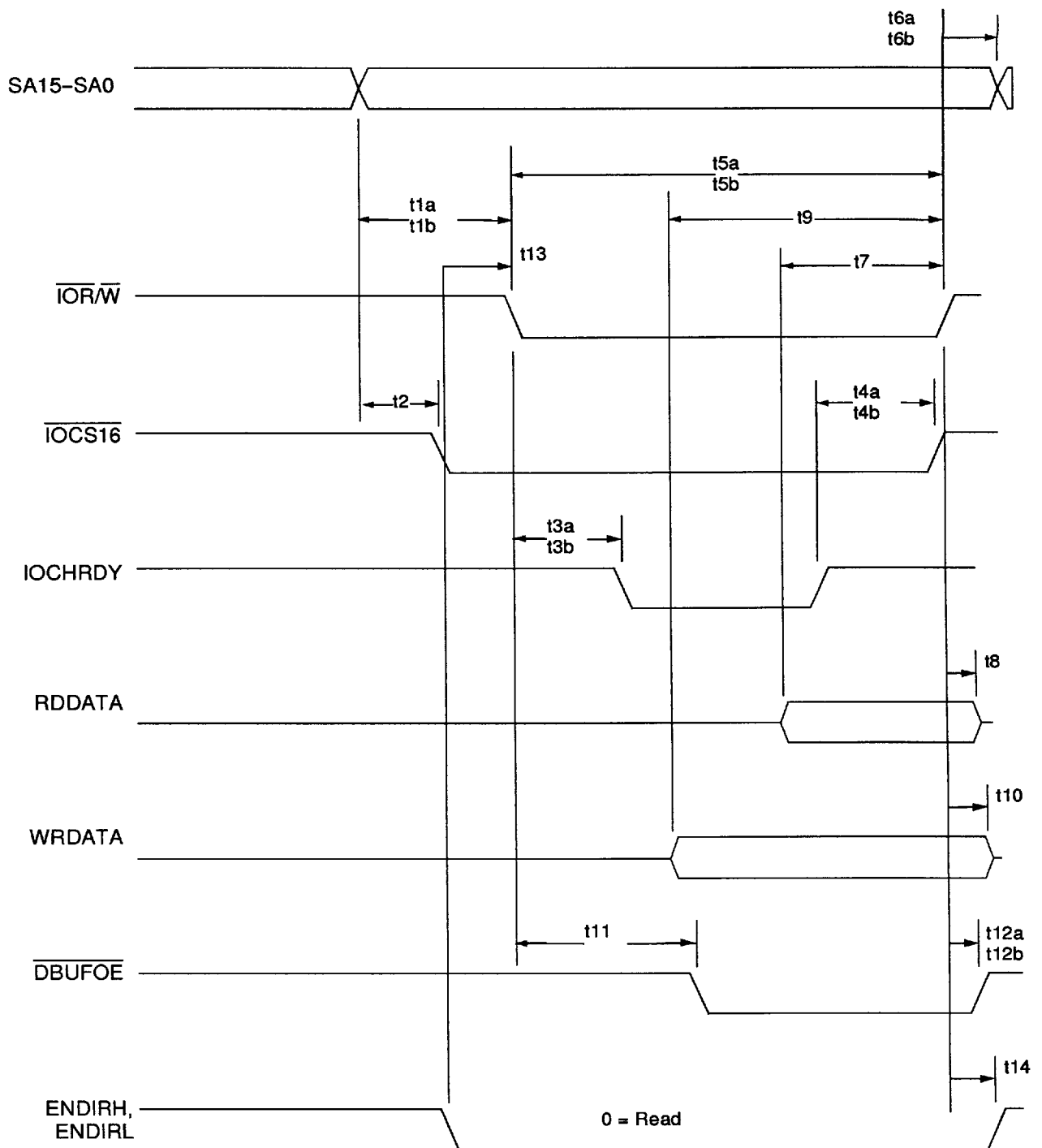
Figure 52. ISA I/O 16-Bit Read/Write Cycle
