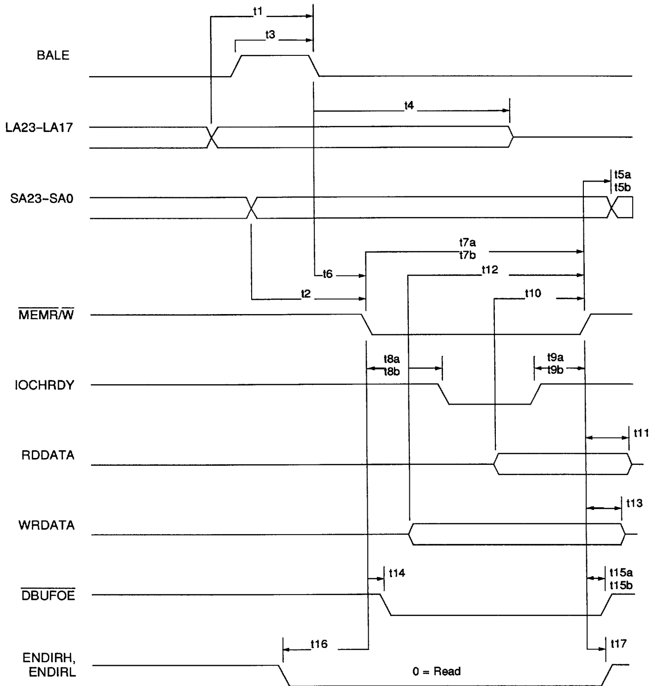
Figure 48. ISA Memory Read/Write 8-Bit Cycle
