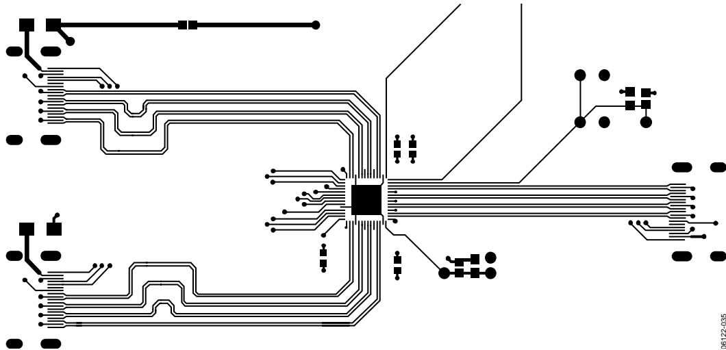
Figure 31. Evaluation Board Layout of the TMD5 Traces
