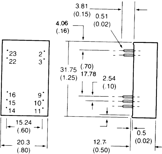
BOTTOM VIEW All dimensions are in mm (inches)
