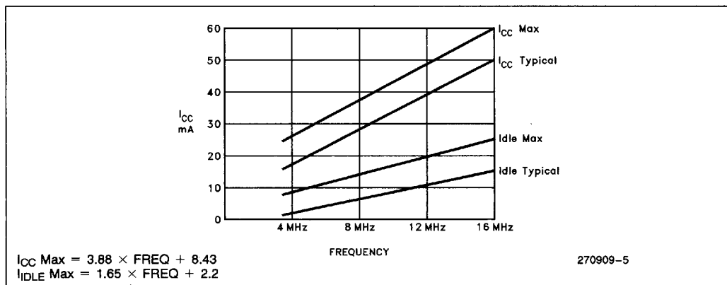
Figure 6. I_{CC} and I_{IDLE} vs Frequency
