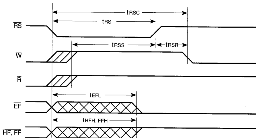
FIGURE 5. RESET TIMING
