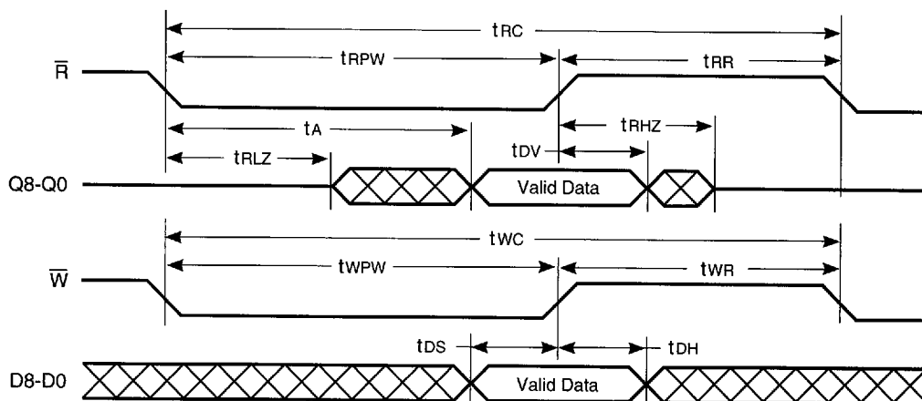
FIGURE 4. ASYNCHRONOUS READ AND WRITE OPERATIONS
