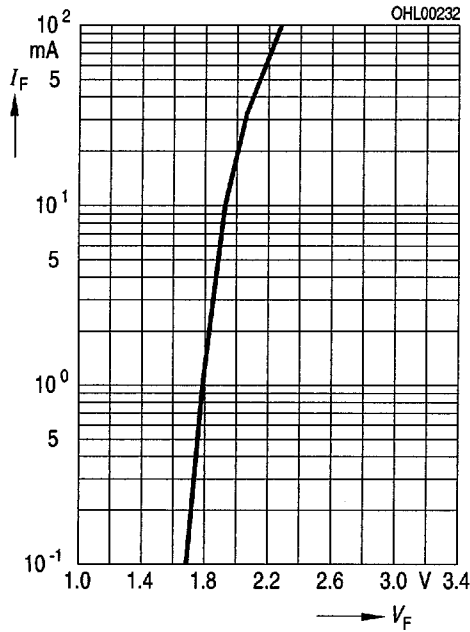
Durchlaßstrom I_F = f(V_F) Forward current T_A = 25^\circ\text{C}
