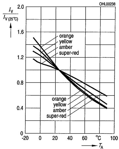
Relative Lichtstärke I_V / I_{V(25^\circ\text{C})} = f(T_A) Relative luminous intensity I_F = 20\text{ mA}
