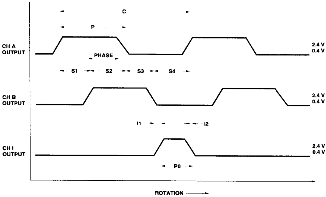
Waveforms for Encoders without Line Drivers.
