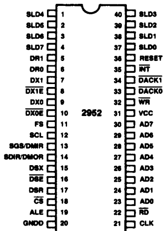
Figure 1. Pin Configuration
