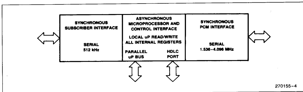
Figure 4. Architectural Diagram
