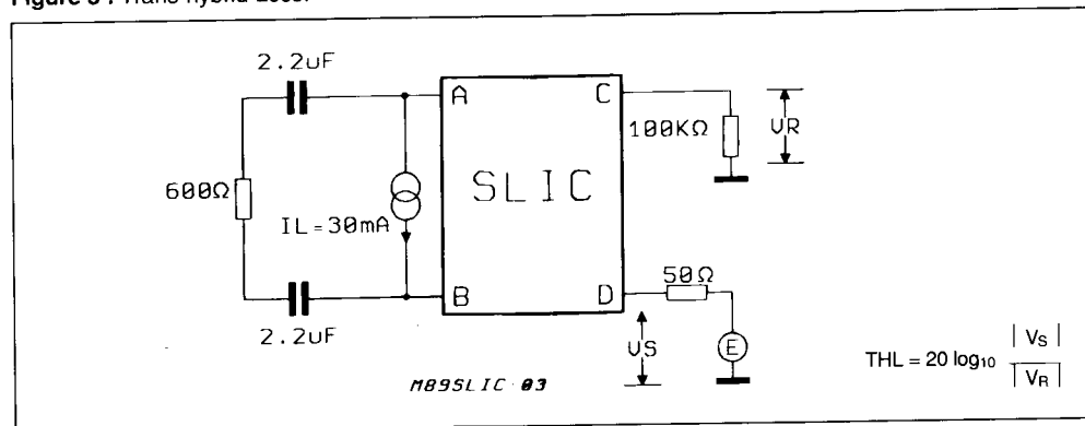
Figure 4 : Sending Gain.
