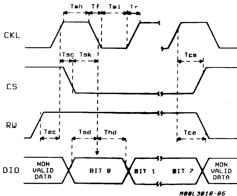
Figure 6 : Writing Operation Timing (from controller to slic).
