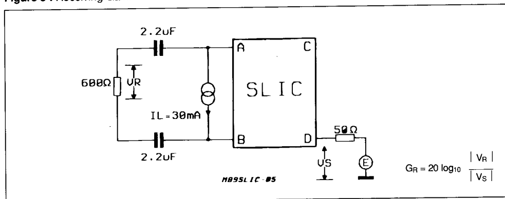
Figure 5 : Receiving Gain.
