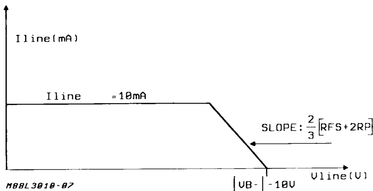
Figure 1 : DC Characteristics in Stand-by Mode.
