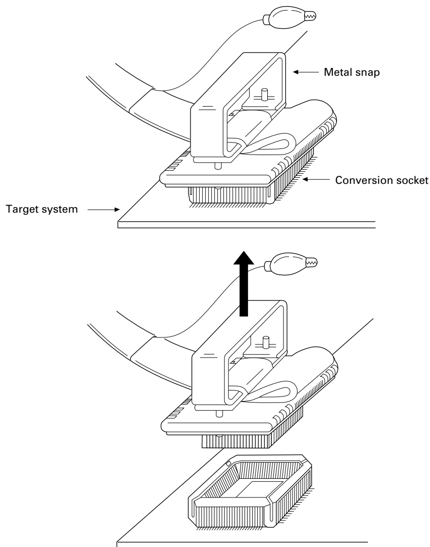
Figure 2-7. Removal of EP-78230GJ-R
